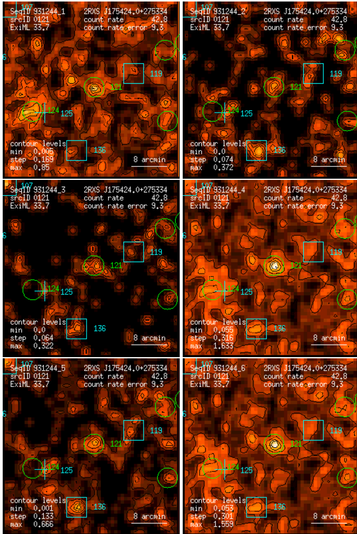
Figure 121: RASS 931244: detection 0121: band rate images, Gaussian filter: (1) PSPC channels 11 – 41, (2) 52 – 90, (3) 91 – 201, (4) 11 – 235, (5) 52 – 201, (6) 11 – 201. Broad band rates in counts/ks. Band rate contour levels in counts/ks/arcmin 2 .
