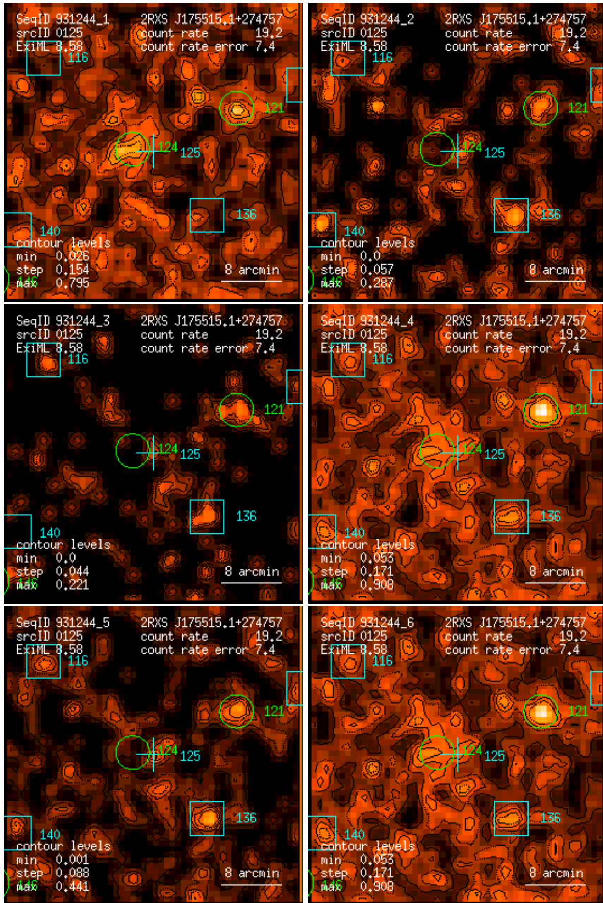
Figure 125: RASS 931244: detection 0125: band rate images, Gaussian filter: (1) PSPC channels 11 – 41, (2) 52 – 90, (3) 91 – 201, (4) 11 – 235, (5) 52 – 201, (6) 11 – 201. Broad band rates in counts/ks. Band rate contour levels in counts/ks/arcmin 2 .
