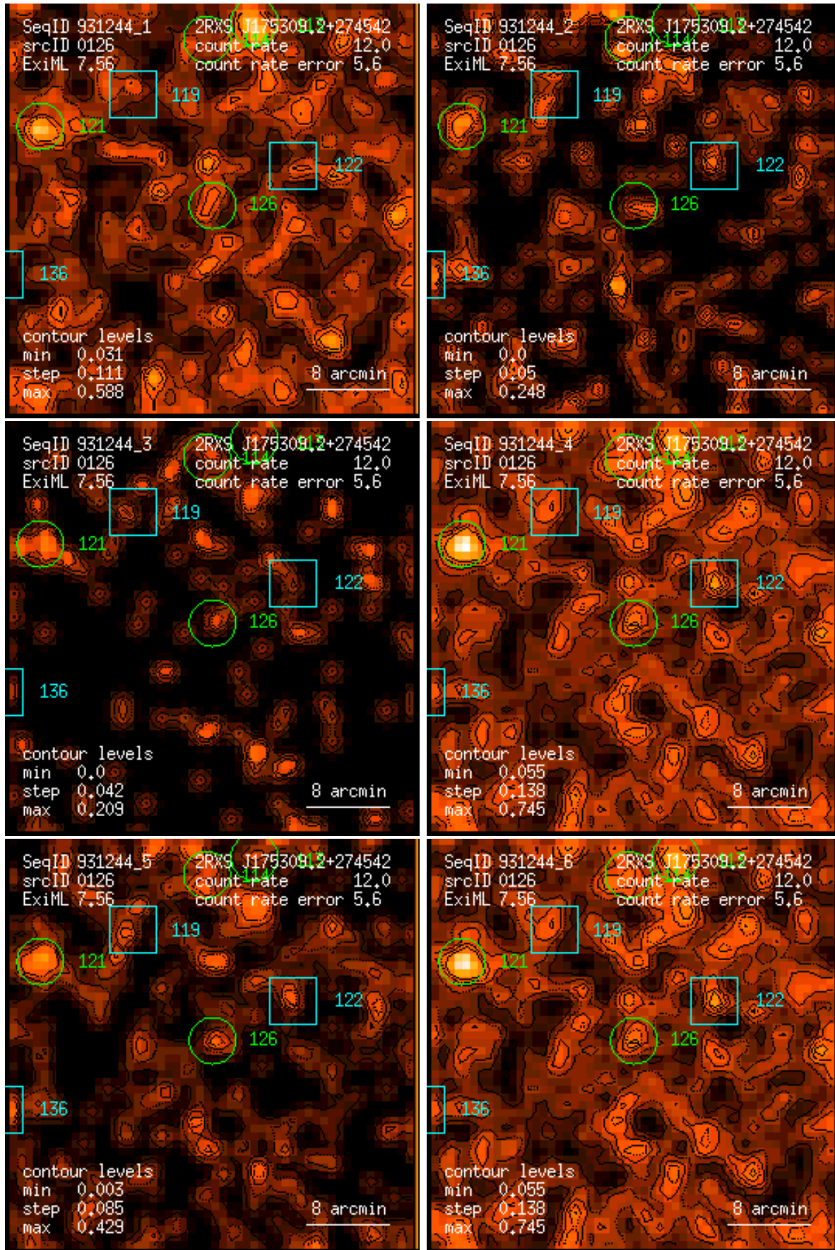
Figure 126: RASS 931244: detection 0126: band rate images, Gaussian filter: (1) PSPC channels 11 – 41, (2) 52 – 90, (3) 91 – 201, (4) 11 – 235, (5) 52 – 201, (6) 11 – 201. Broad band rates in counts/ks. Band rate contour levels in counts/ks/arcmin 2 .
