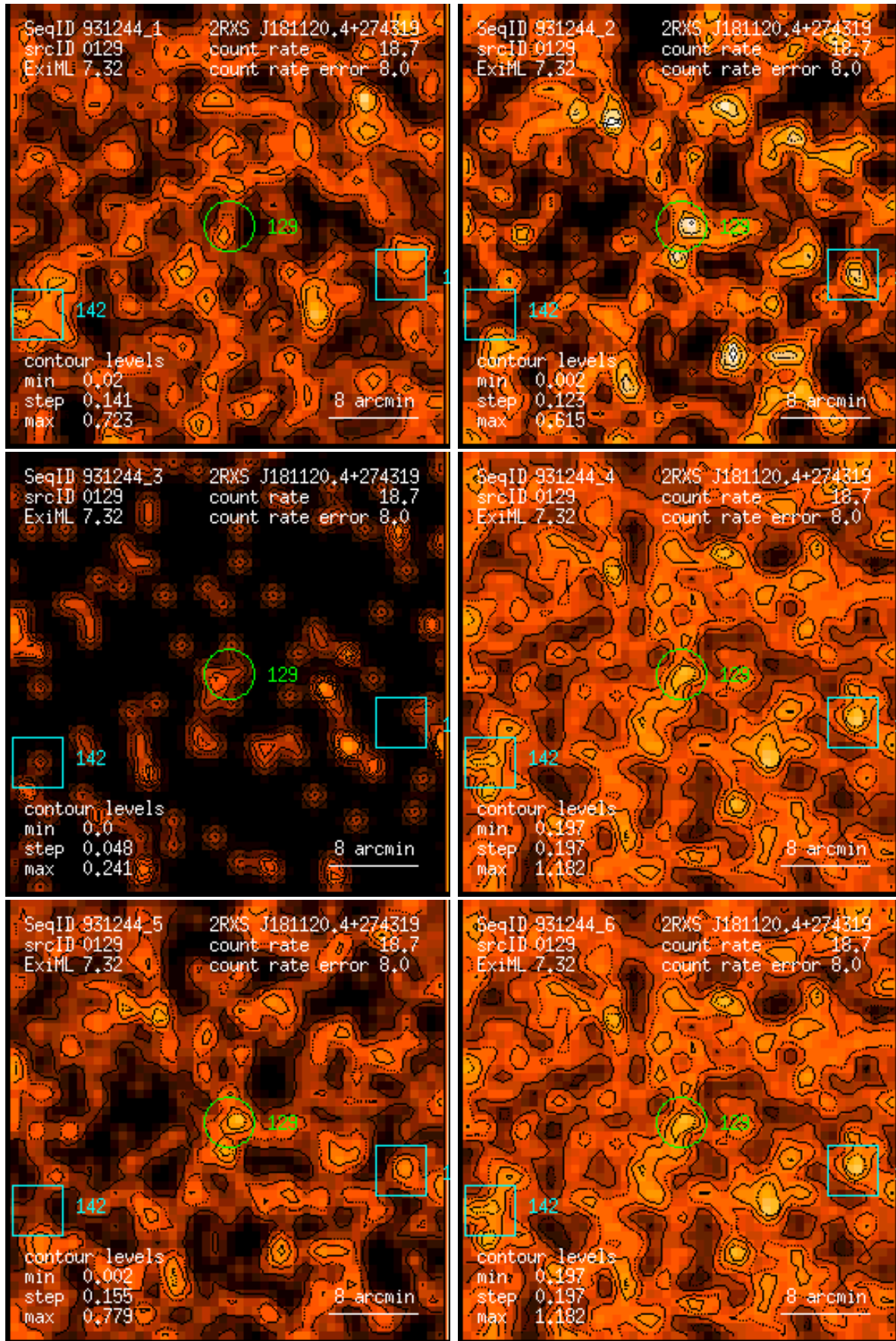
Figure 129: RASS 931244: detection 0129: band rate images, Gaussian filter: (1) PSPC channels 11 – 41, (2) 52 – 90, (3) 91 – 201, (4) 11 – 235, (5) 52 – 201, (6) 11 – 201. Broad band rates in counts/ks. Band rate contour levels in counts/ks/arcmin 2 .
