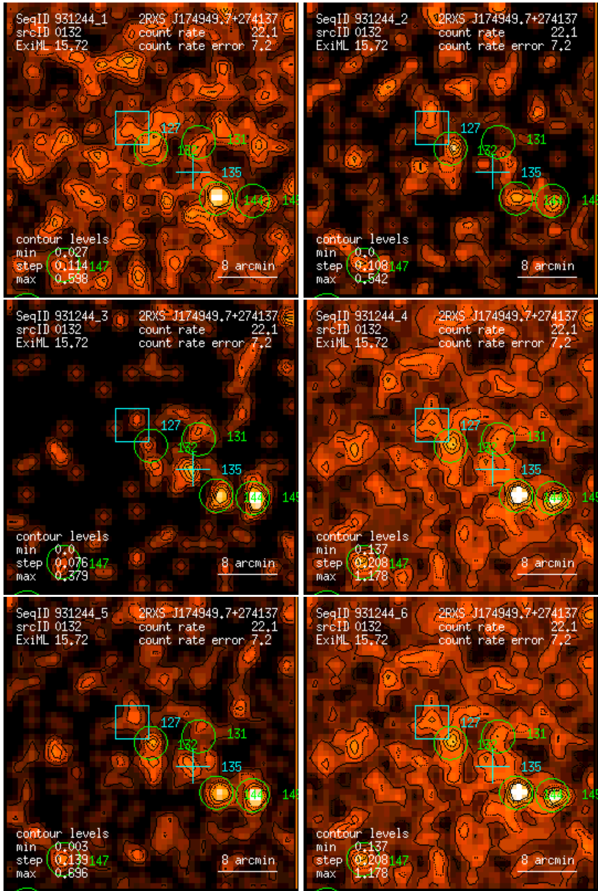
Figure 132: RASS 931244: detection 0132: band rate images, Gaussian filter: (1) PSPC channels 11 – 41, (2) 52 – 90, (3) 91 – 201, (4) 11 – 235, (5) 52 – 201, (6) 11 – 201. Broad band rates in counts/ks. Band rate contour levels in counts/ks/arcmin 2 .
