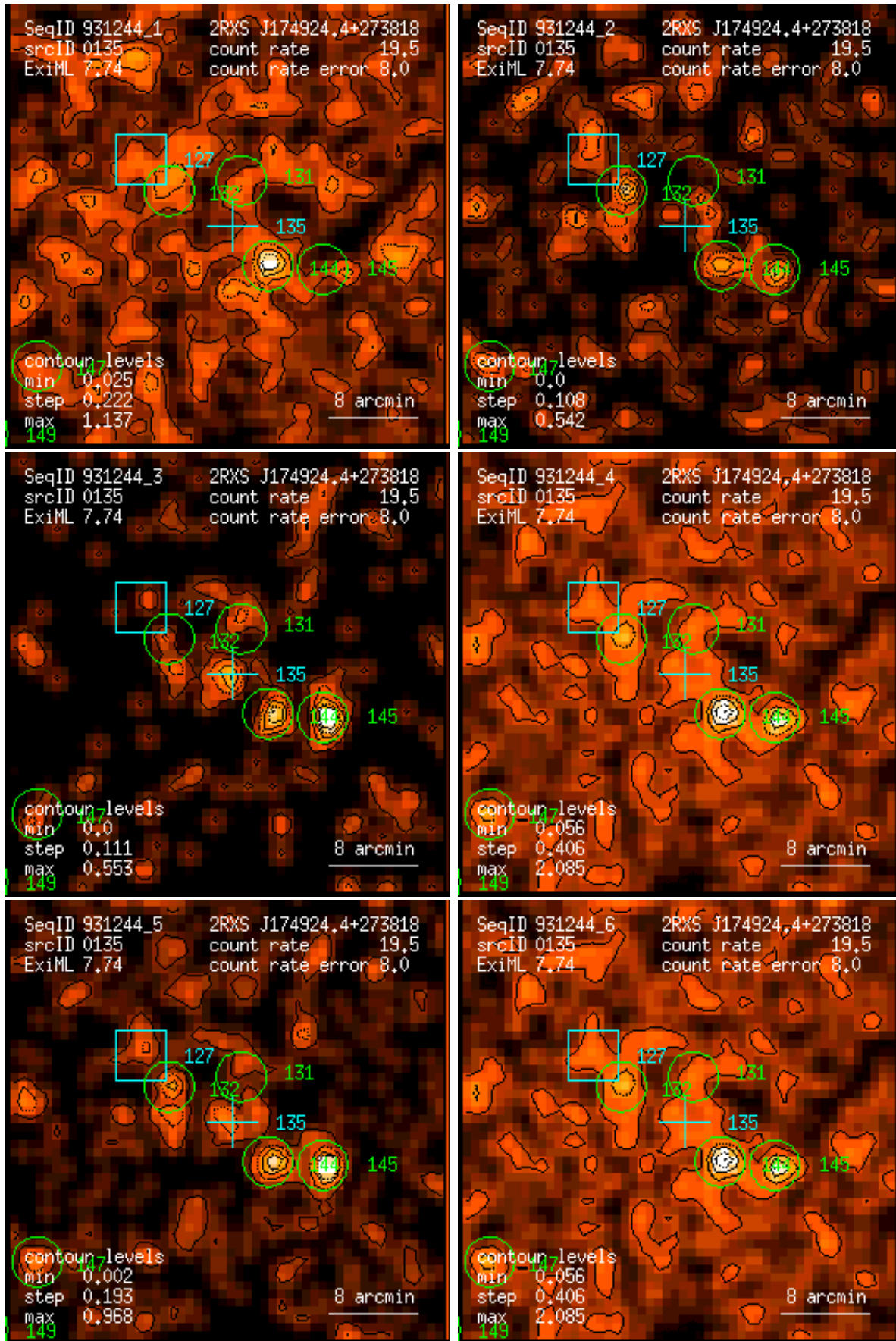
Figure 135: RASS 931244: detection 0135: band rate images, Gaussian filter: (1) PSPC channels 11 – 41, (2) 52 – 90, (3) 91 – 201, (4) 11 – 235, (5) 52 – 201, (6) 11 – 201. Broad band rates in counts/ks. Band rate contour levels in counts/ks/arcmin 2 .
