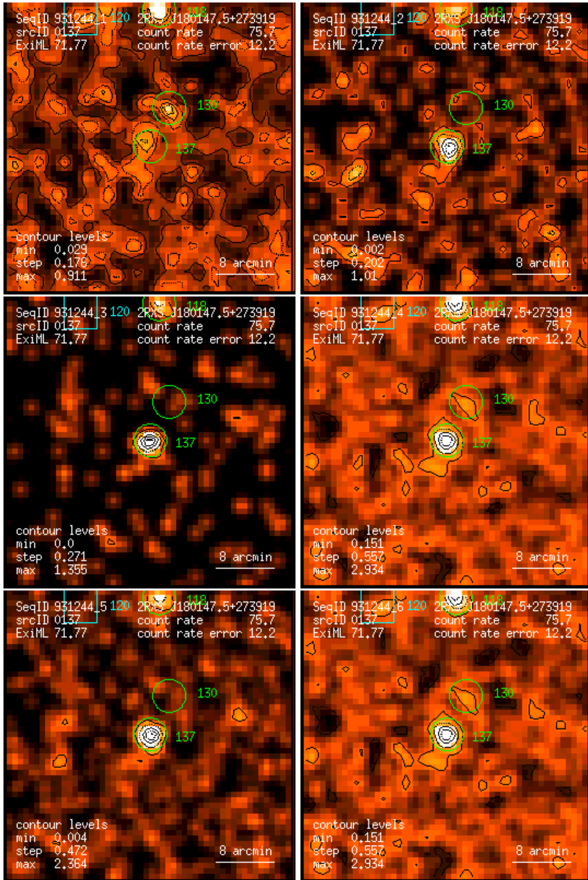
Figure 137: RASS 931244: detection 0137: band rate images, Gaussian filter: (1) PSPC channels 11 – 41, (2) 52 – 90, (3) 91 – 201, (4) 11 – 235, (5) 52 – 201, (6) 11 – 201. Broad band rates in counts/ks. Band rate contour levels in counts/ks/arcmin 2 .
