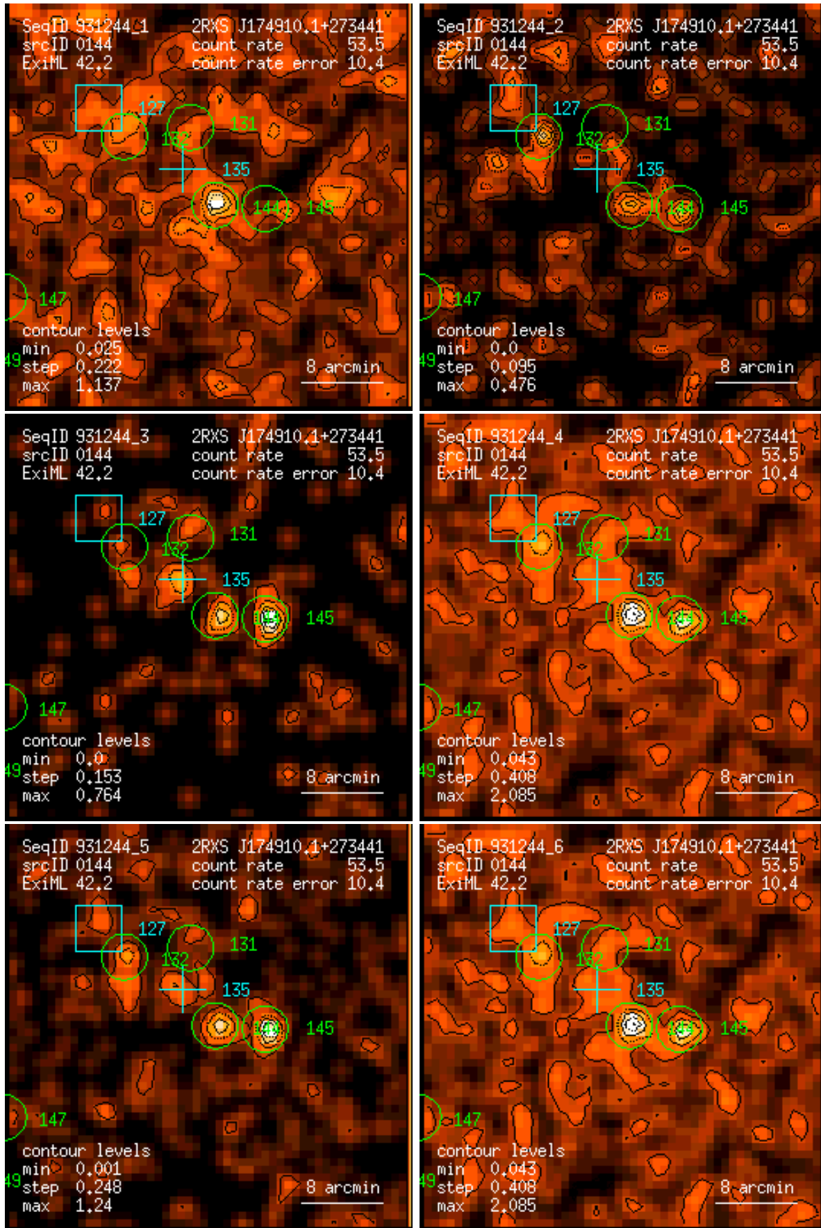
Figure 144: RASS 931244: detection 0144: band rate images, Gaussian filter: (1) PSPC channels 11 – 41, (2) 52 – 90, (3) 91 – 201, (4) 11 – 235, (5) 52 – 201, (6) 11 – 201. Broad band rates in counts/ks. Band rate contour levels in counts/ks/arcmin 2 .
