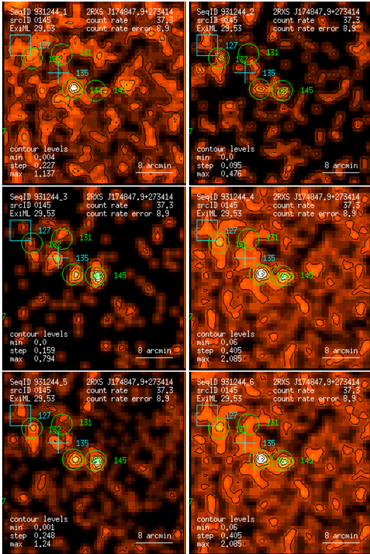
Figure 145: RASS 931244: detection 0145: band rate images, Gaussian filter: (1) PSPC channels 11 – 41, (2) 52 – 90, (3) 91 – 201, (4) 11 – 235, (5) 52 – 201, (6) 11 – 201. Broad band rates in counts/ks. Band rate contour levels in counts/ks/arcmin 2 .
