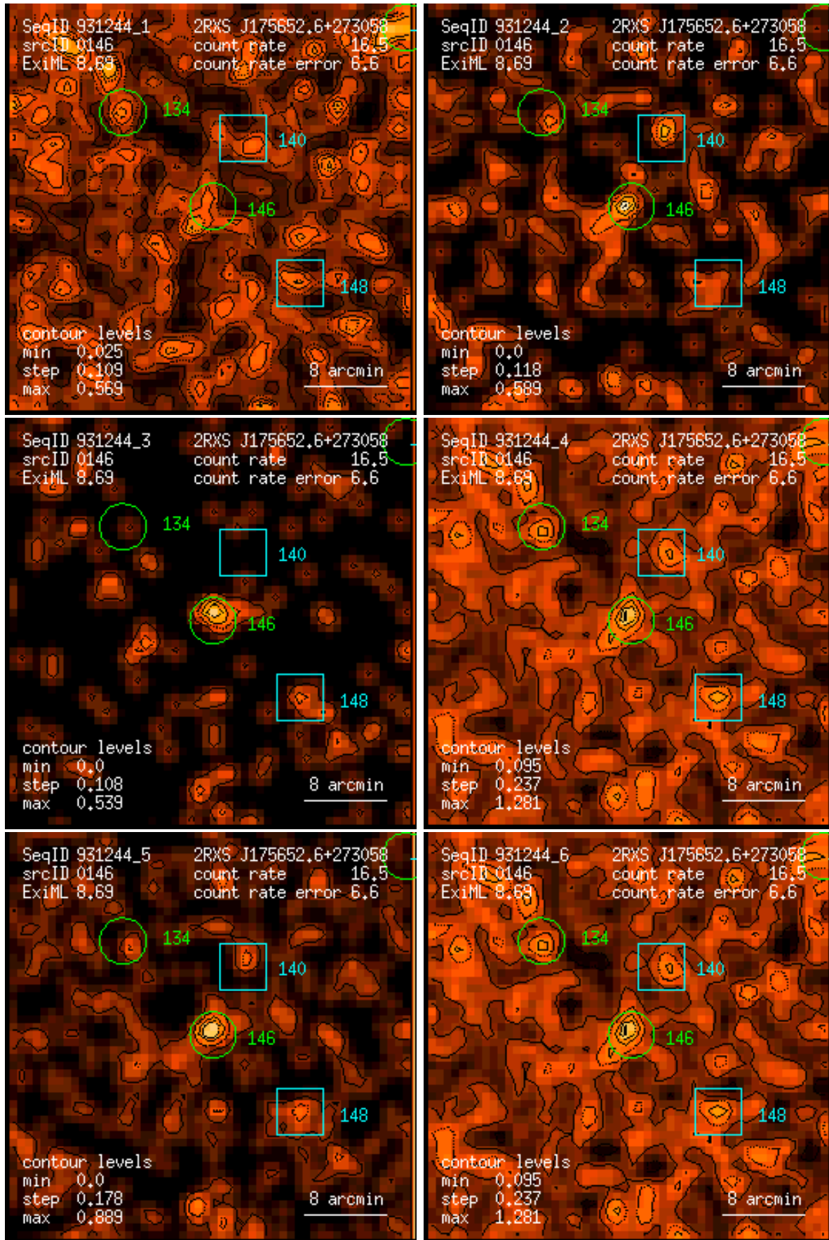
Figure 146: RASS 931244: detection 0146: band rate images, Gaussian filter: (1) PSPC channels 11 – 41, (2) 52 – 90, (3) 91 – 201, (4) 11 – 235, (5) 52 – 201, (6) 11 – 201. Broad band rates in counts/ks. Band rate contour levels in counts/ks/arcmin 2 .
