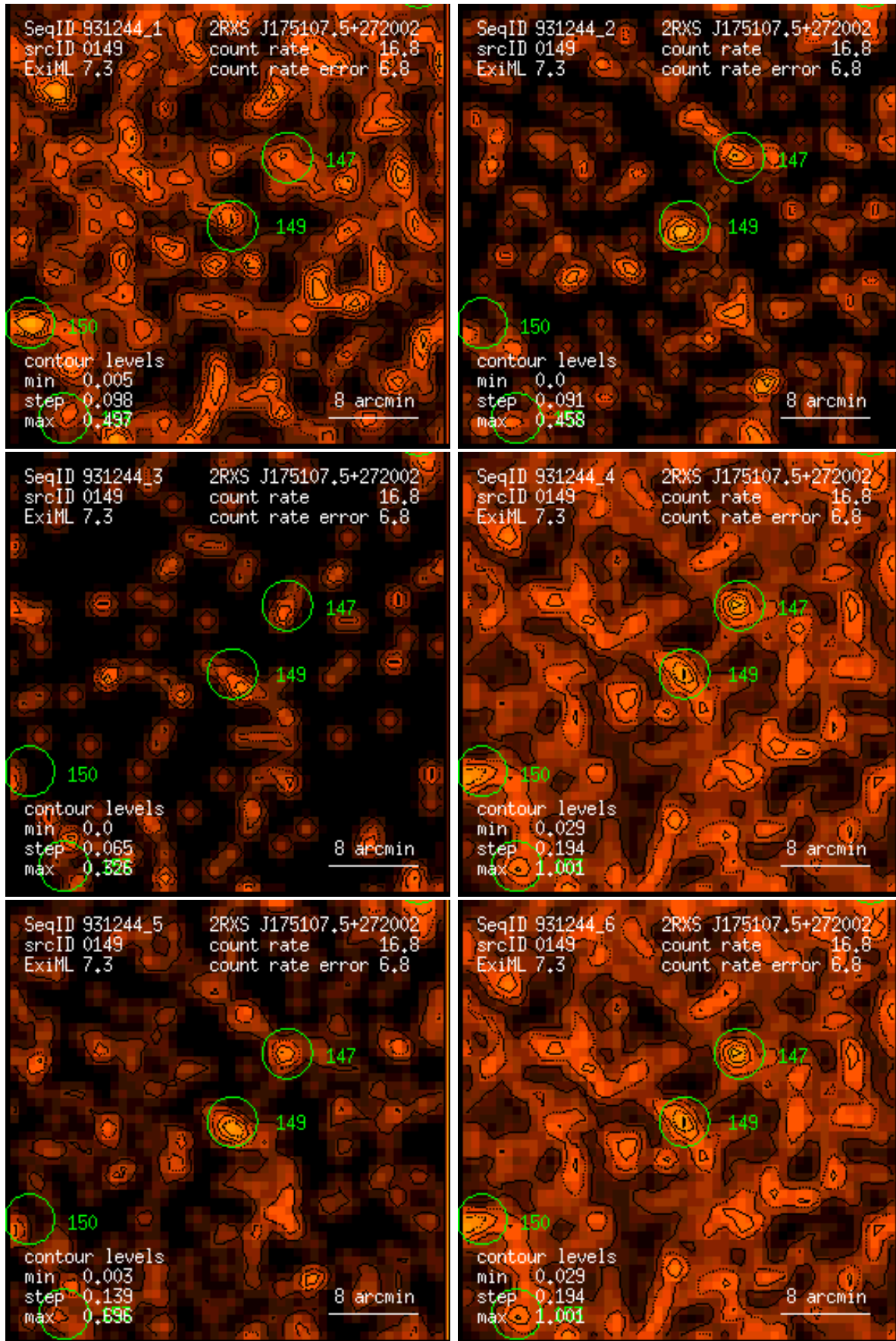
Figure 149: RASS 931244: detection 0149: band rate images, Gaussian filter: (1) PSPC channels 11 – 41, (2) 52 – 90, (3) 91 – 201, (4) 11 – 235, (5) 52 – 201, (6) 11 – 201. Broad band rates in counts/ks. Band rate contour levels in counts/ks/arcmin 2 .
