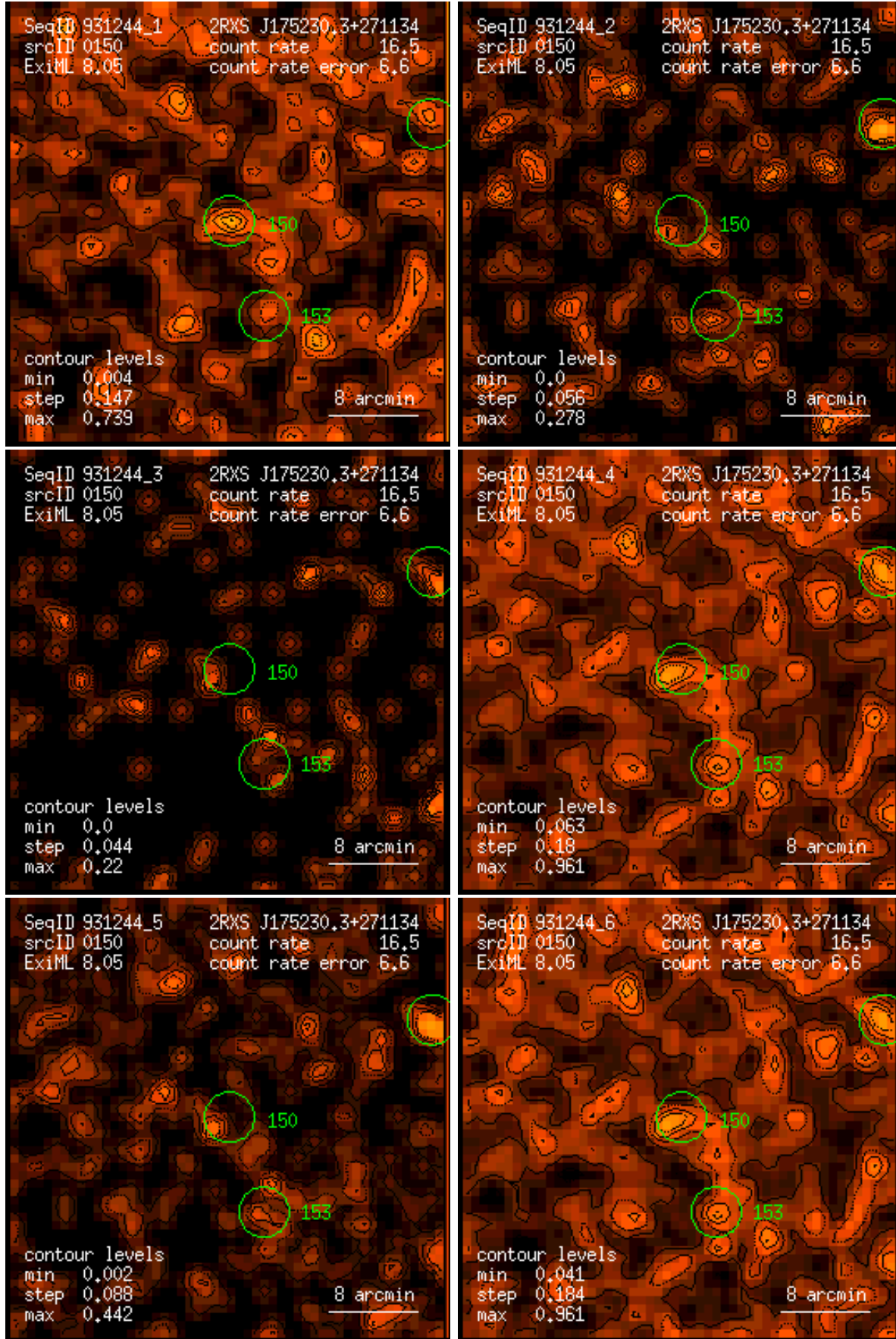
Figure 150: RASS 931244: detection 0150: band rate images, Gaussian filter: (1) PSPC channels 11 – 41, (2) 52 – 90, (3) 91 – 201, (4) 11 – 235, (5) 52 – 201, (6) 11 – 201. Broad band rates in counts/ks. Band rate contour levels in counts/ks/arcmin 2 .
