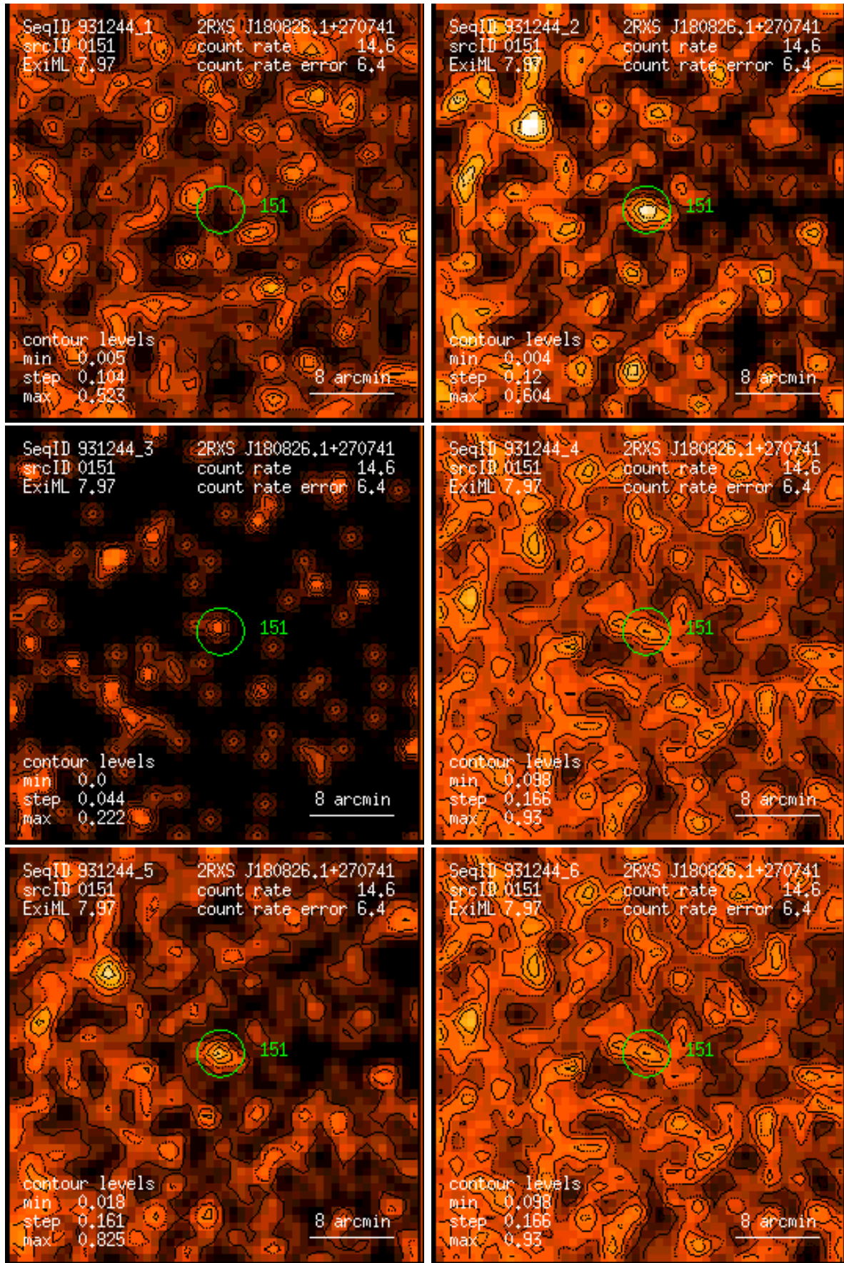
Figure 151: RASS 931244: detection 0151: band rate images, Gaussian filter: (1) PSPC channels 11 – 41, (2) 52 – 90, (3) 91 – 201, (4) 11 – 235, (5) 52 – 201, (6) 11 – 201. Broad band rates in counts/ks. Band rate contour levels in counts/ks/arcmin 2 .
