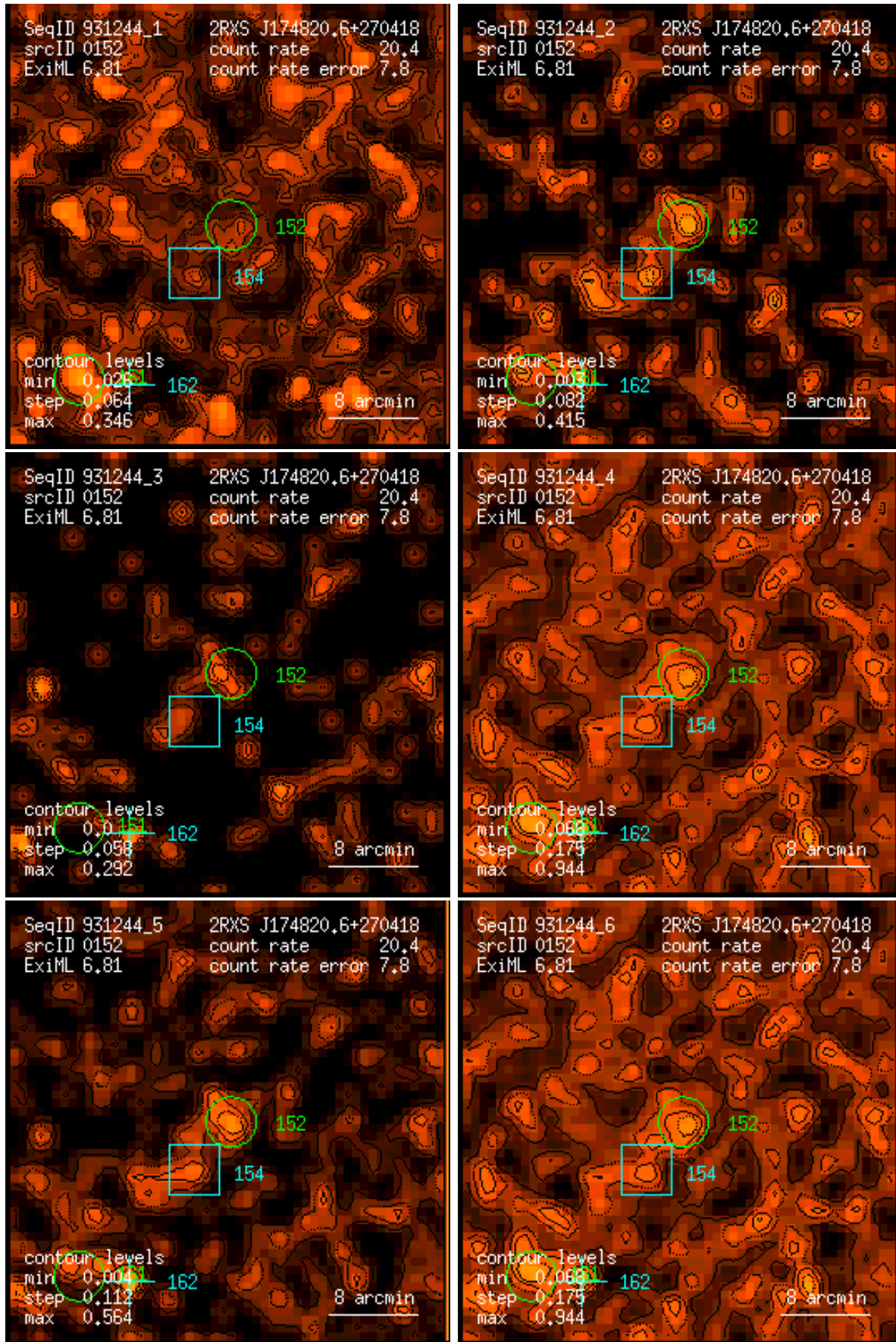
Figure 152: RASS 931244: detection 0152: band rate images, Gaussian filter: (1) PSPC channels 11 – 41, (2) 52 – 90, (3) 91 – 201, (4) 11 – 235, (5) 52 – 201, (6) 11 – 201. Broad band rates in counts/ks. Band rate contour levels in counts/ks/arcmin 2 .
