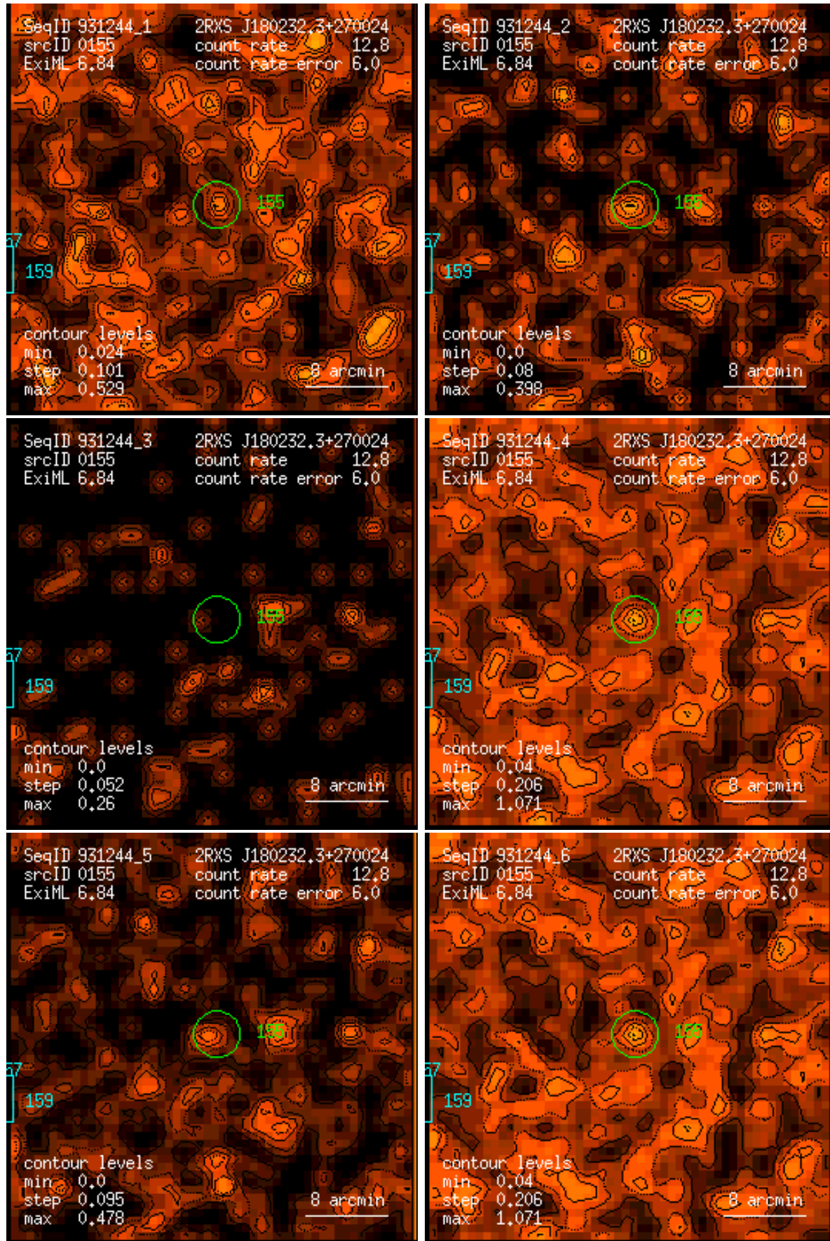
Figure 155: RASS 931244: detection 0155: band rate images, Gaussian filter: (1) PSPC channels 11 – 41, (2) 52 – 90, (3) 91 – 201, (4) 11 – 235, (5) 52 – 201, (6) 11 – 201. Broad band rates in counts/ks. Band rate contour levels in counts/ks/arcmin 2 .
