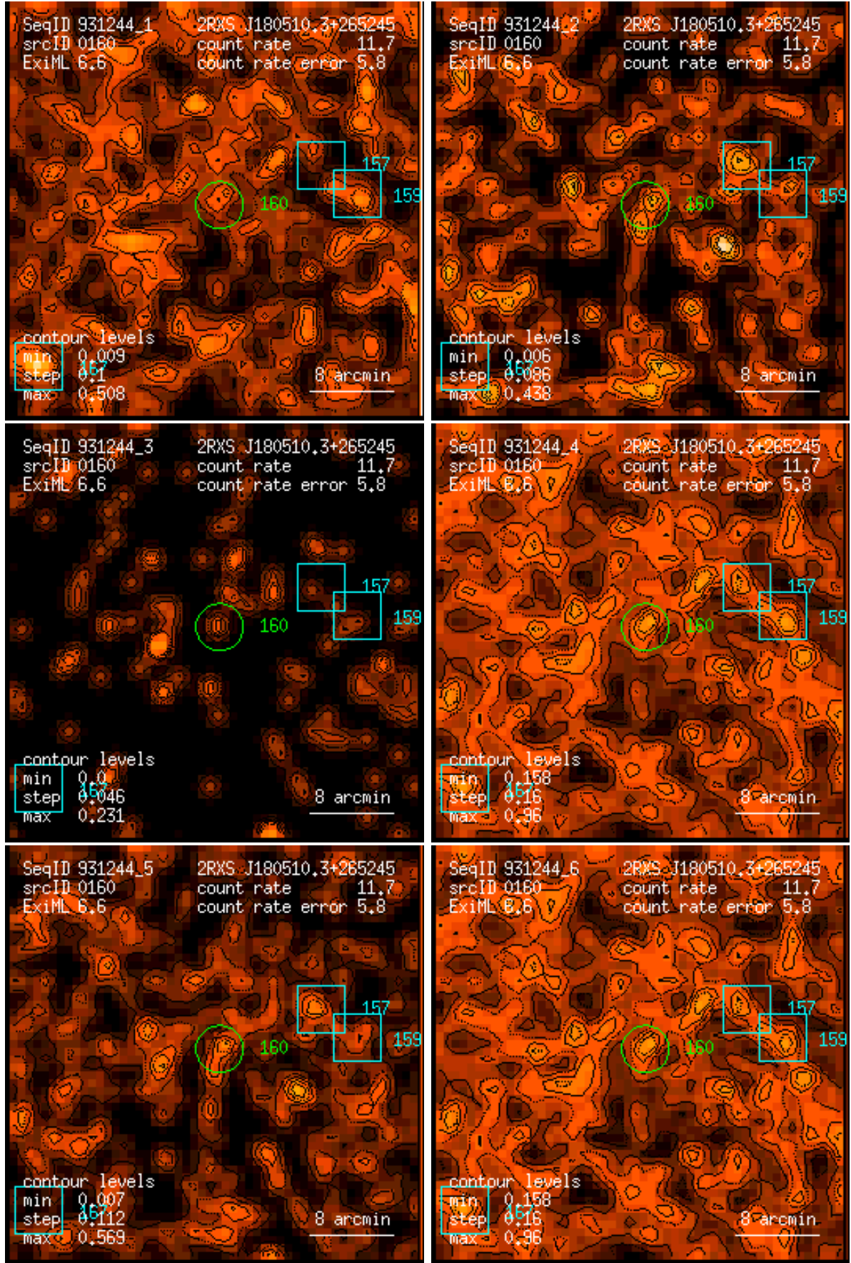
Figure 160: RASS 931244: detection 0160: band rate images, Gaussian filter: (1) PSPC channels 11 – 41, (2) 52 – 90, (3) 91 – 201, (4) 11 – 235, (5) 52 – 201, (6) 11 – 201. Broad band rates in counts/ks. Band rate contour levels in counts/ks/arcmin 2 .
