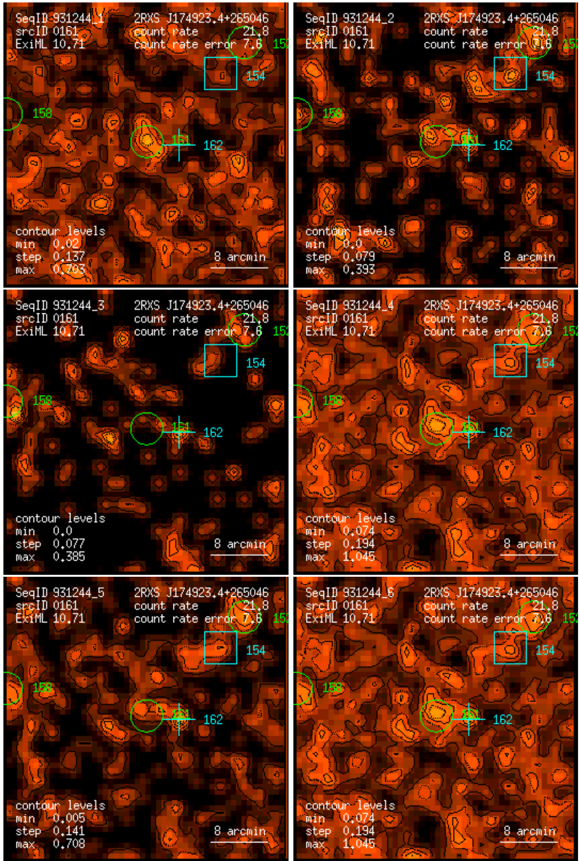
Figure 161: RASS 931244: detection 0161: band rate images, Gaussian filter: (1) PSPC channels 11 – 41, (2) 52 – 90, (3) 91 – 201, (4) 11 – 235, (5) 52 – 201, (6) 11 – 201. Broad band rates in counts/ks. Band rate contour levels in counts/ks/arcmin 2 .
