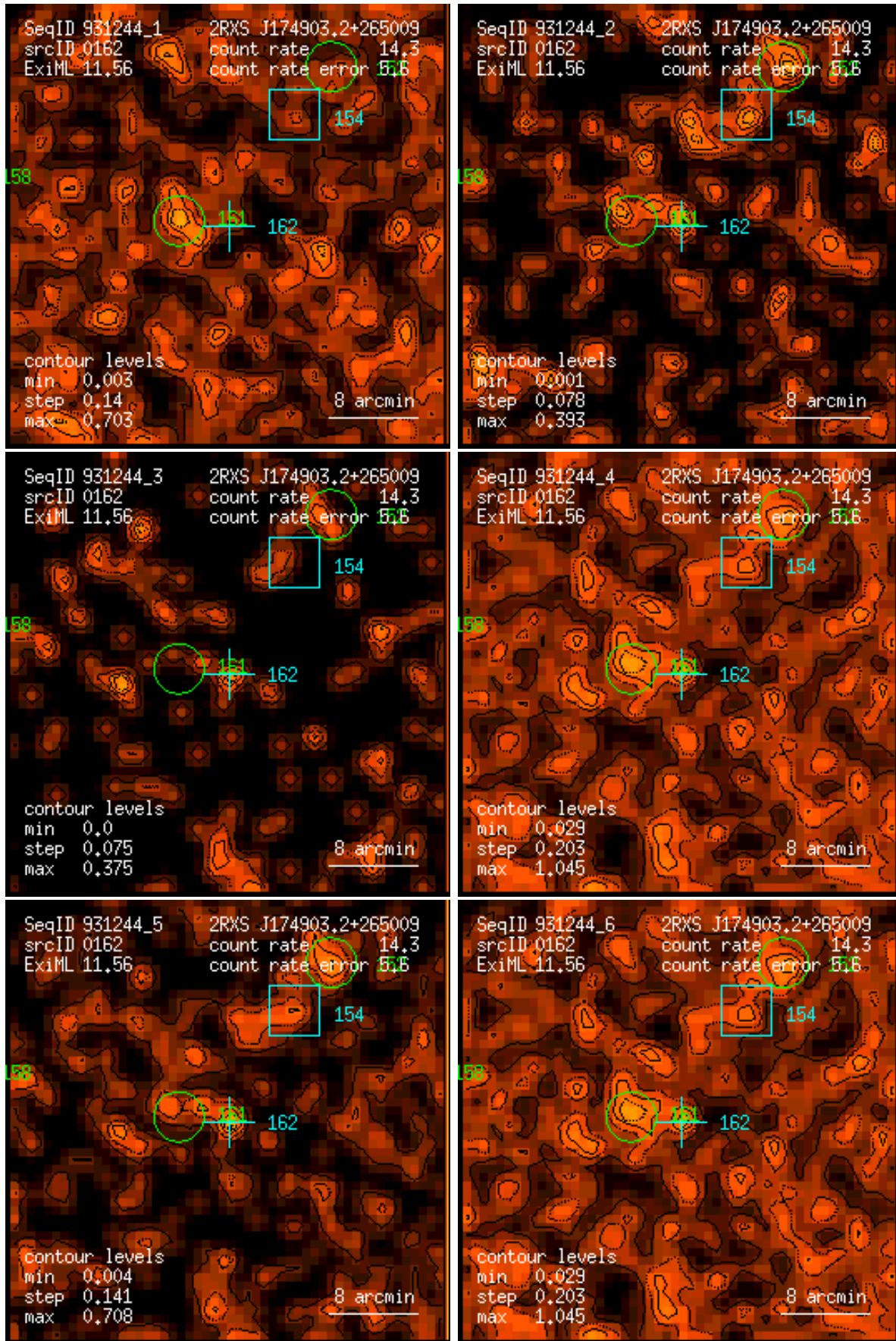
Figure 162: RASS 931244: detection 0162: band rate images, Gaussian filter: (1) PSPC channels 11 – 41, (2) 52 – 90, (3) 91 – 201, (4) 11 – 235, (5) 52 – 201, (6) 11 – 201. Broad band rates in counts/ks. Band rate contour levels in counts/ks/arcmin 2 .
