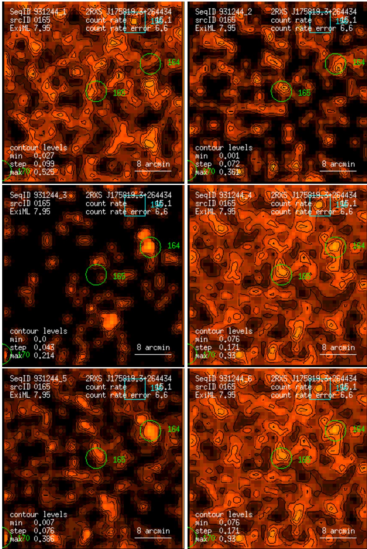
Figure 165: RASS 931244: detection 0165: band rate images, Gaussian filter: (1) PSPC channels 11 – 41, (2) 52 – 90, (3) 91 – 201, (4) 11 – 235, (5) 52 – 201, (6) 11 – 201. Broad band rates in counts/ks. Band rate contour levels in counts/ks/arcmin 2 .
