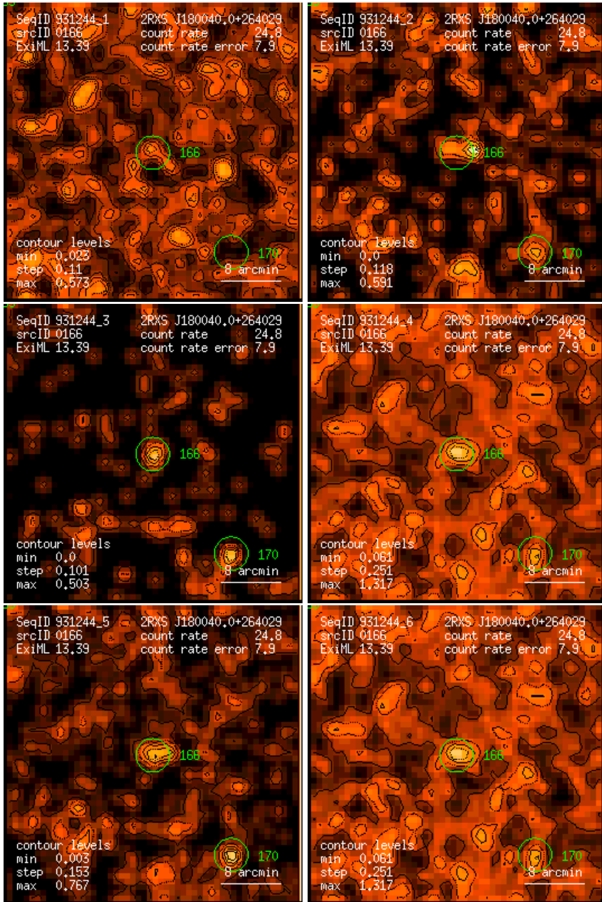
Figure 166: RASS 931244: detection 0166: band rate images, Gaussian filter: (1) PSPC channels 11 – 41, (2) 52 – 90, (3) 91 – 201, (4) 11 – 235, (5) 52 – 201, (6) 11 – 201. Broad band rates in counts/ks. Band rate contour levels in counts/ks/arcmin 2 .
