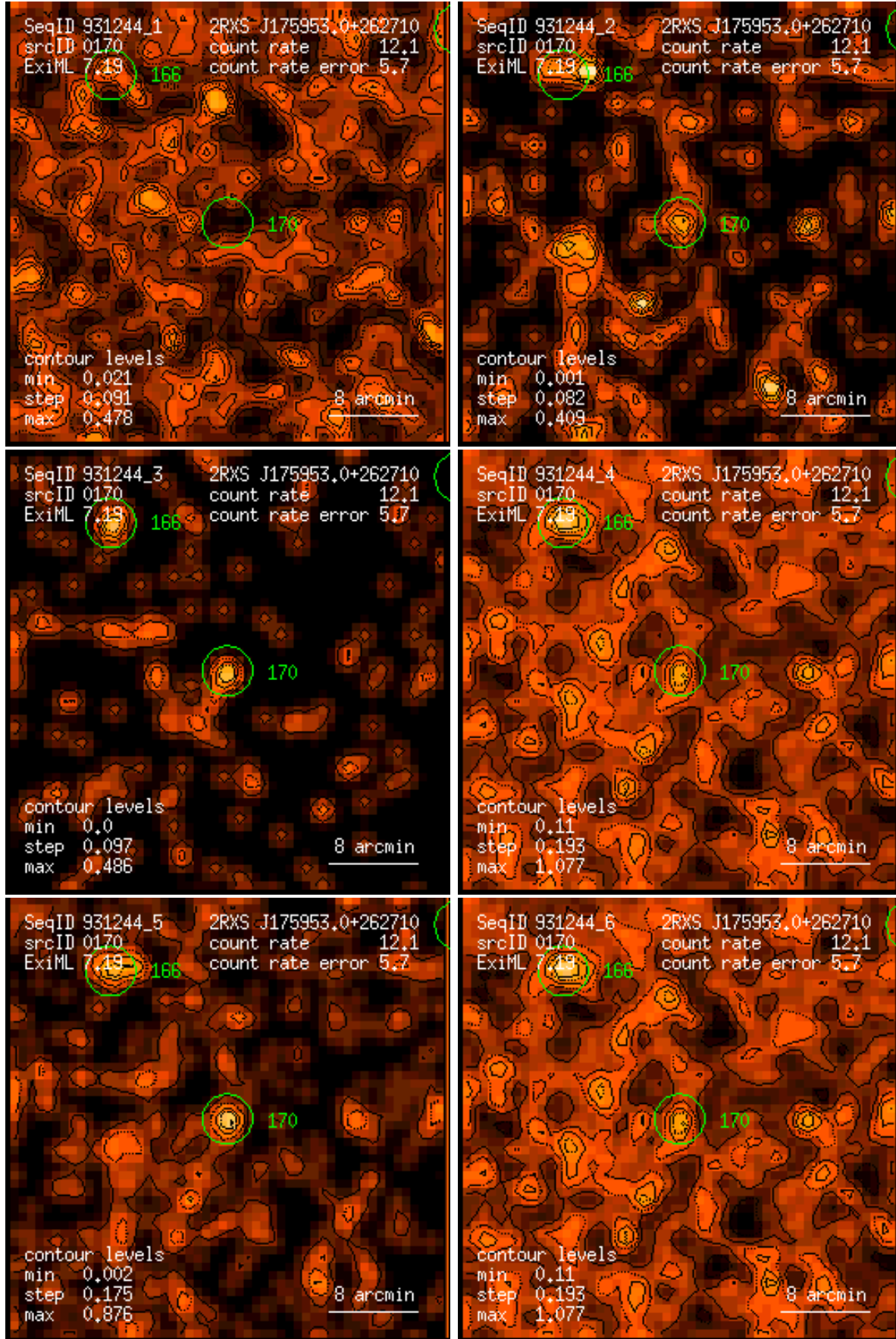
Figure 170: RASS 931244: detection 0170: band rate images, Gaussian filter: (1) PSPC channels 11 – 41, (2) 52 – 90, (3) 91 – 201, (4) 11 – 235, (5) 52 – 201, (6) 11 – 201. Broad band rates in counts/ks. Band rate contour levels in counts/ks/arcmin 2 .
