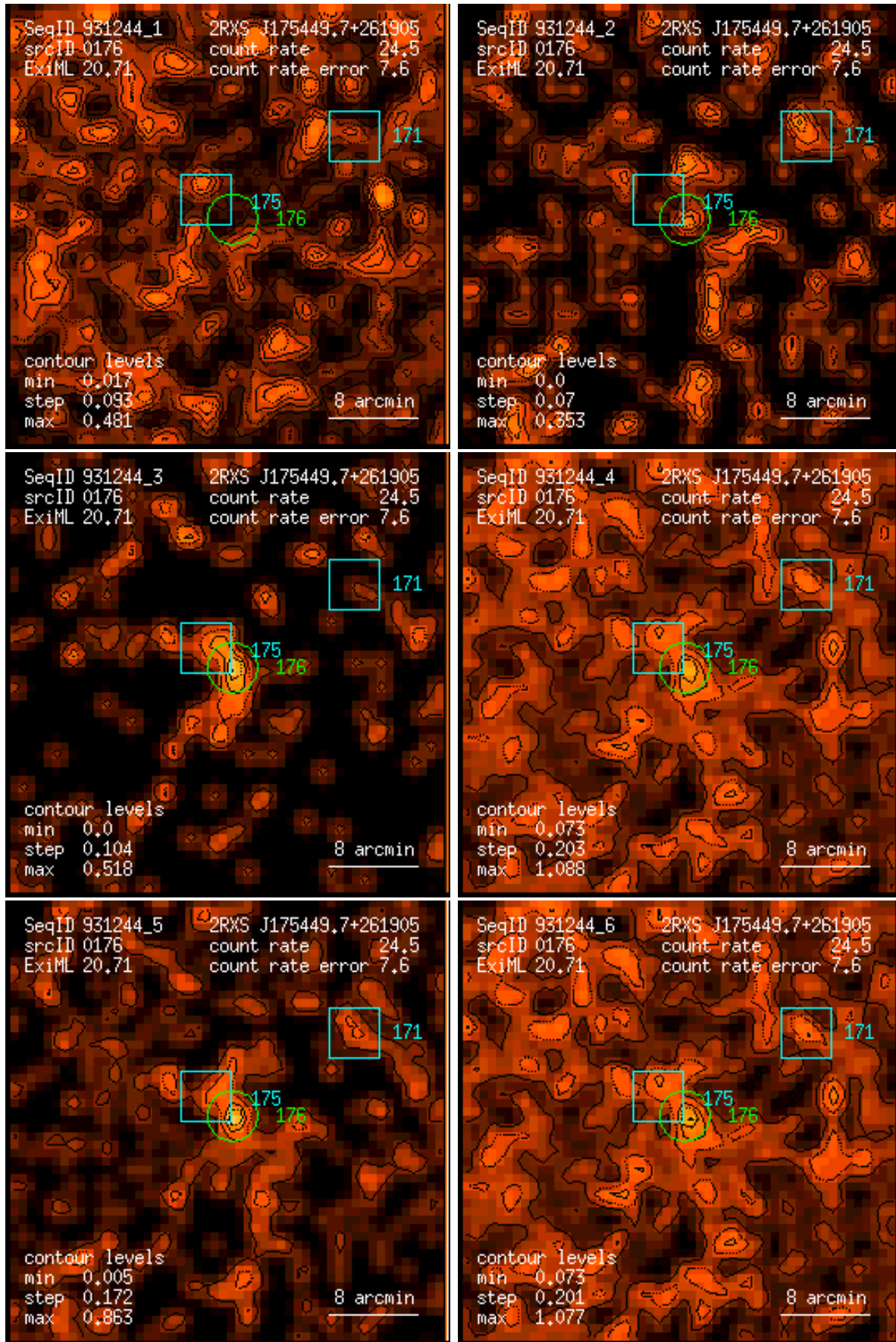
Figure 176: RASS 931244: detection 0176: band rate images, Gaussian filter: (1) PSPC channels 11 – 41, (2) 52 – 90, (3) 91 – 201, (4) 11 – 235, (5) 52 – 201, (6) 11 – 201. Broad band rates in counts/ks. Band rate contour levels in counts/ks/arcmin 2 .
