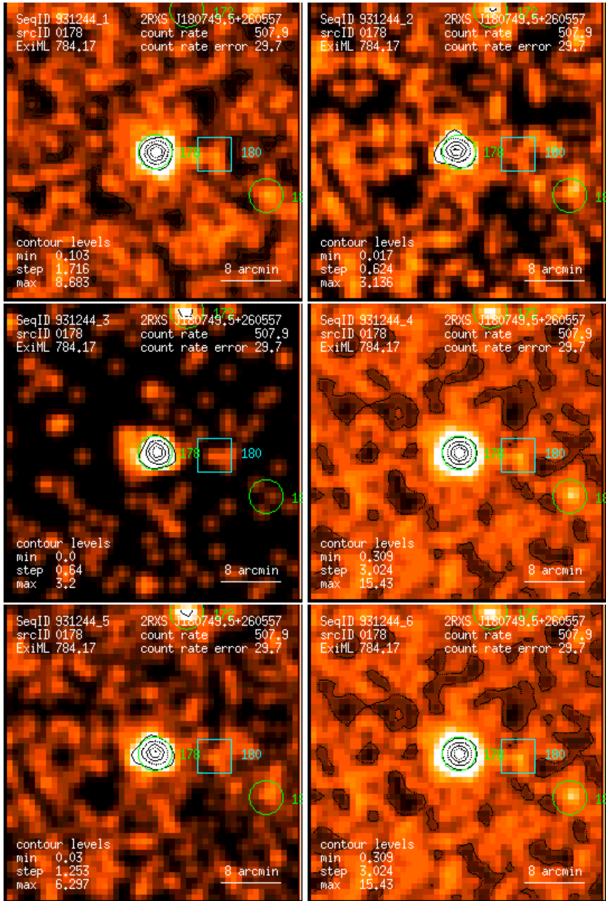
Figure 178: RASS 931244: detection 0178: band rate images, Gaussian filter: (1) PSPC channels 11 – 41, (2) 52 – 90, (3) 91 – 201, (4) 11 – 235, (5) 52 – 201, (6) 11 – 201. Broad band rates in counts/ks. Band rate contour levels in counts/ks/arcmin 2 .
