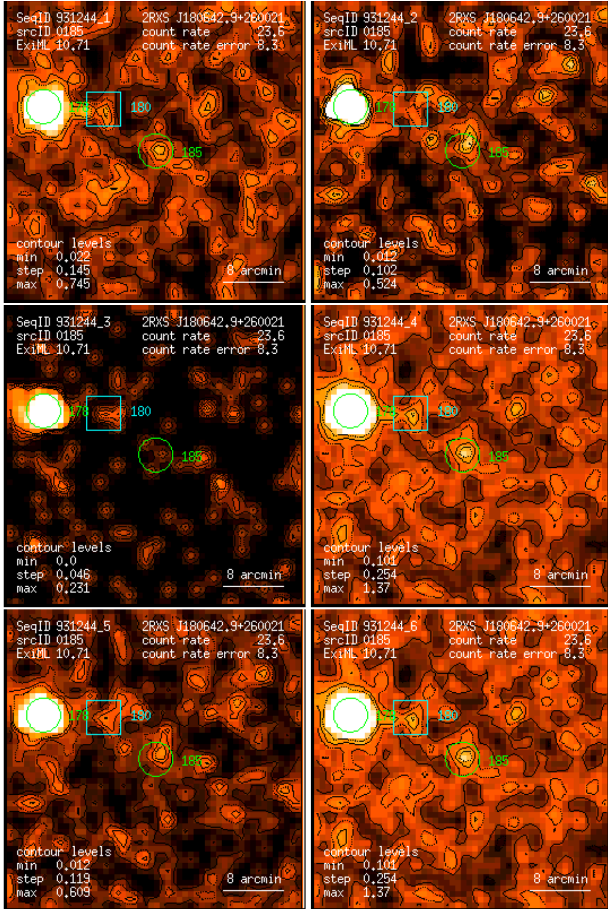
Figure 185: RASS 931244: detection 0185: band rate images, Gaussian filter: (1) PSPC channels 11 – 41, (2) 52 – 90, (3) 91 – 201, (4) 11 – 235, (5) 52 – 201, (6) 11 – 201. Broad band rates in counts/ks. Band rate contour levels in counts/ks/arcmin 2 .
