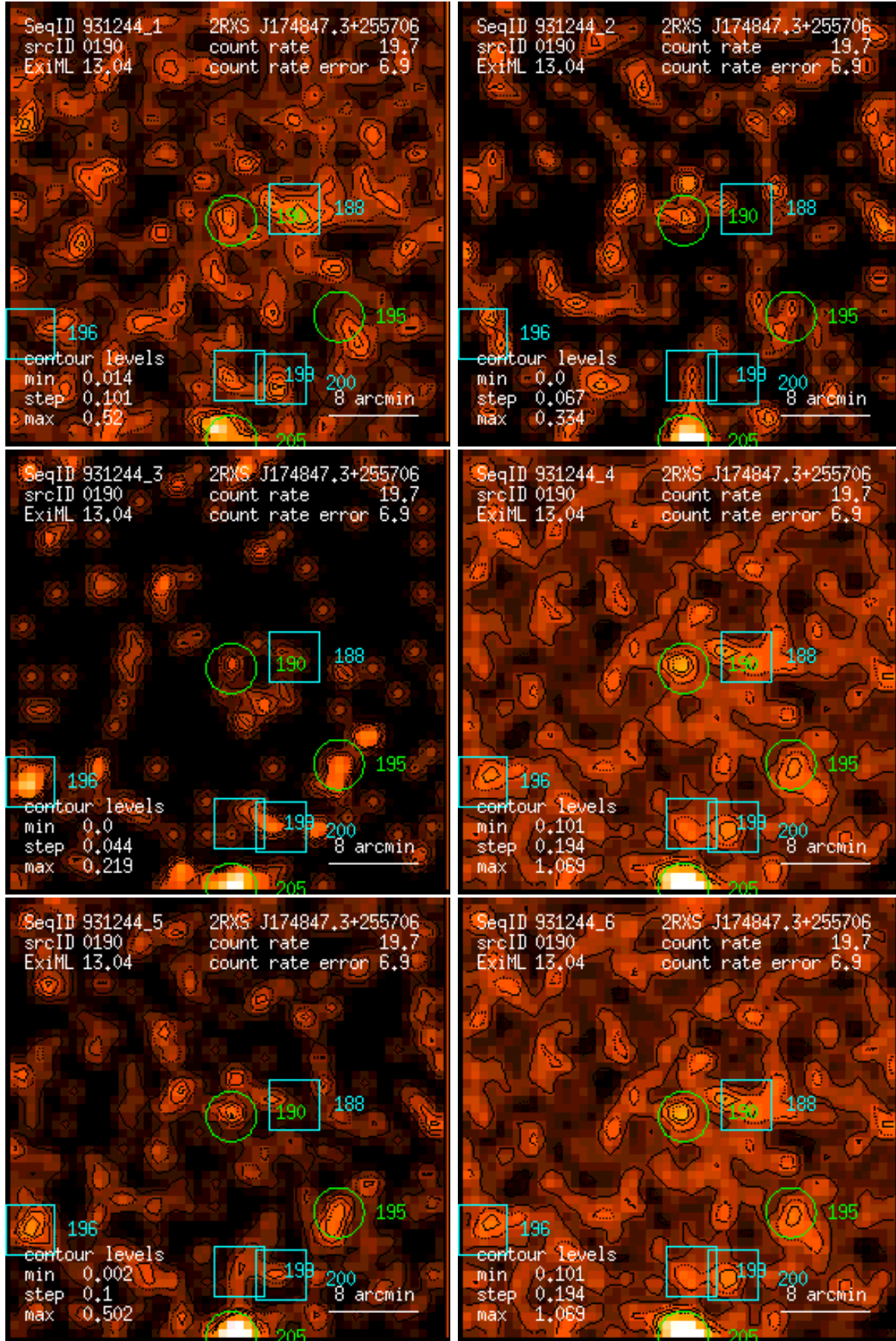
Figure 190: RASS 931244: detection 0190: band rate images, Gaussian filter: (1) PSPC channels 11 – 41, (2) 52 – 90, (3) 91 – 201, (4) 11 – 235, (5) 52 – 201, (6) 11 – 201. Broad band rates in counts/ks. Band rate contour levels in counts/ks/arcmin 2 .
