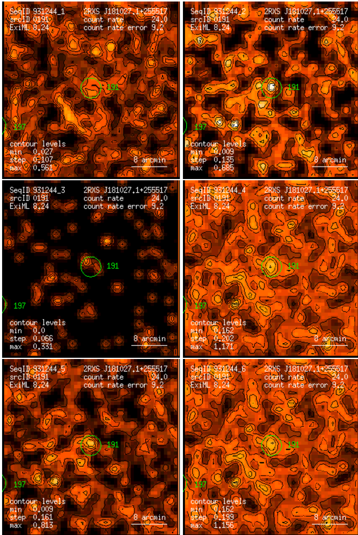
Figure 191: RASS 931244: detection 0191: band rate images, Gaussian filter: (1) PSPC channels 11 – 41, (2) 52 – 90, (3) 91 – 201, (4) 11 – 235, (5) 52 – 201, (6) 11 – 201. Broad band rates in counts/ks. Band rate contour levels in counts/ks/arcmin 2 .
