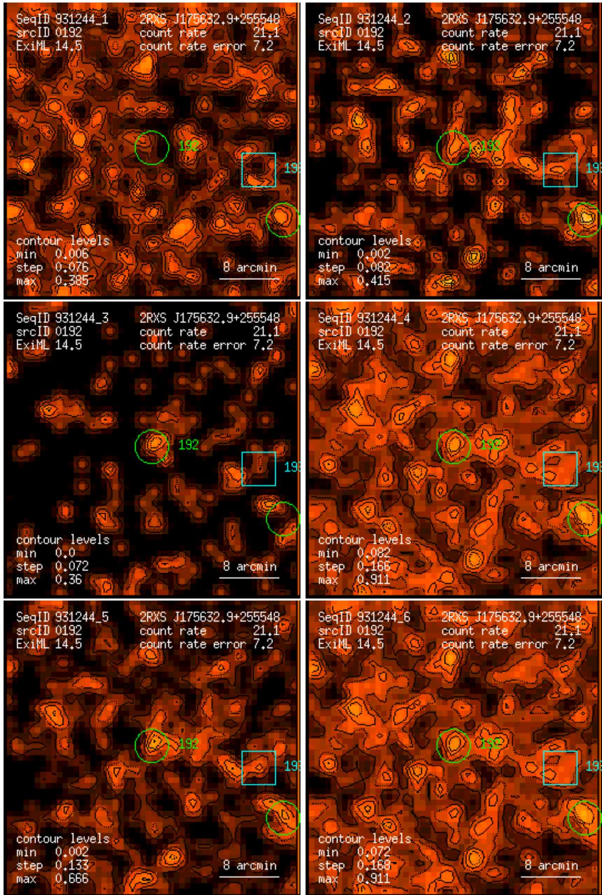
Figure 192: RASS 931244: detection 0192: band rate images, Gaussian filter: (1) PSPC channels 11 – 41, (2) 52 – 90, (3) 91 – 201, (4) 11 – 235, (5) 52 – 201, (6) 11 – 201. Broad band rates in counts/ks. Band rate contour levels in counts/ks/arcmin 2 .
