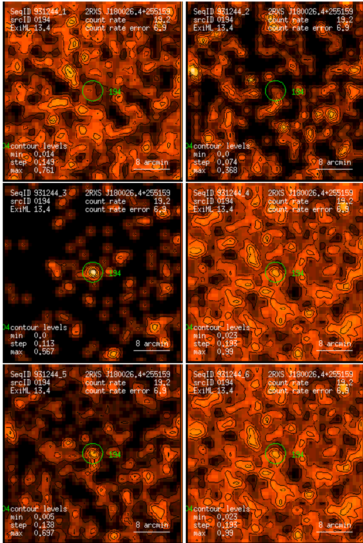
Figure 194: RASS 931244: detection 0194: band rate images, Gaussian filter: (1) PSPC channels 11 – 41, (2) 52 – 90, (3) 91 – 201, (4) 11 – 235, (5) 52 – 201, (6) 11 – 201. Broad band rates in counts/ks. Band rate contour levels in counts/ks/arcmin 2 .
