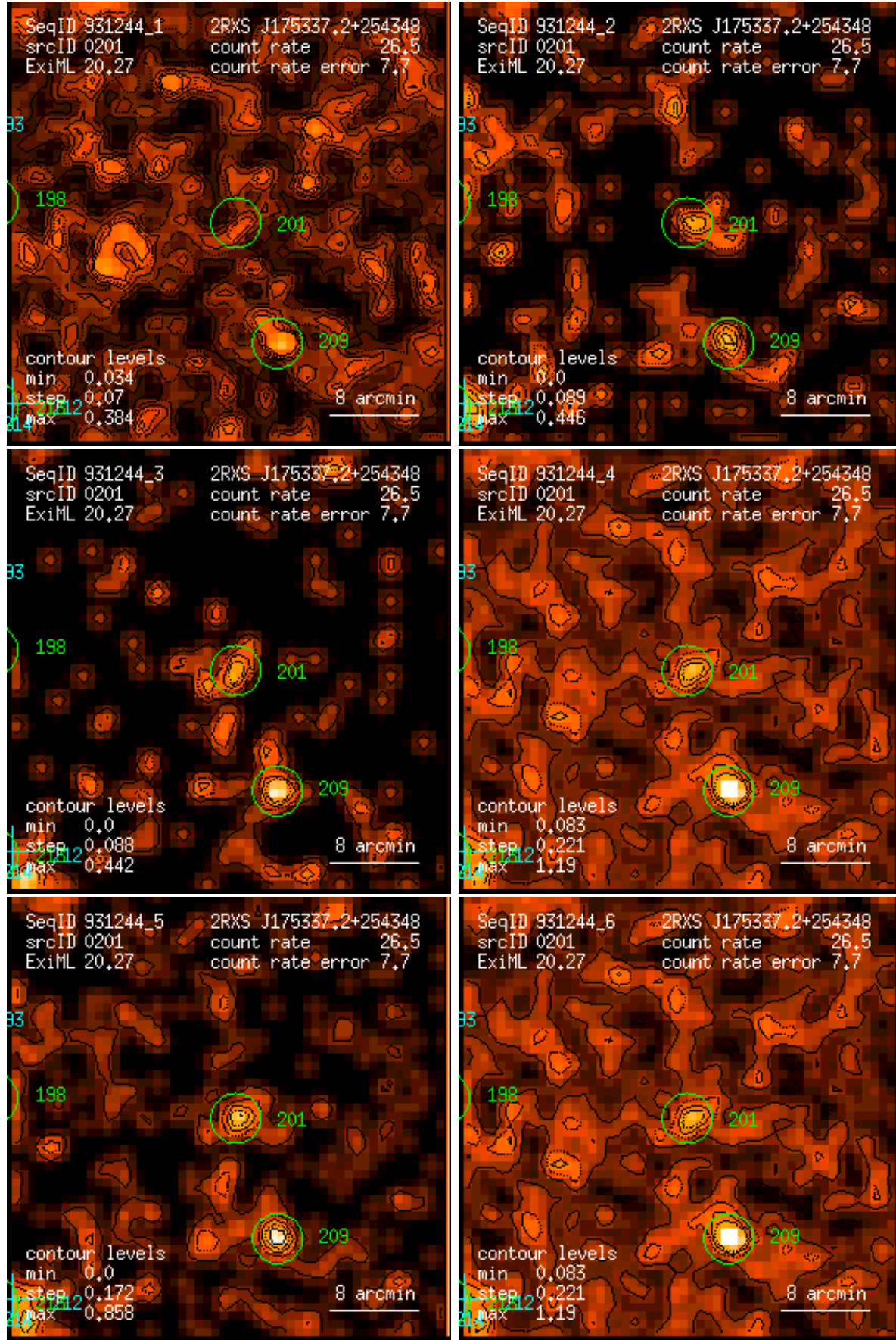
Figure 201: RASS 931244: detection 0201: band rate images, Gaussian filter: (1) PSPC channels 11 – 41, (2) 52 – 90, (3) 91 – 201, (4) 11 – 235, (5) 52 – 201, (6) 11 – 201. Broad band rates in counts/ks. Band rate contour levels in counts/ks/arcmin 2 .
