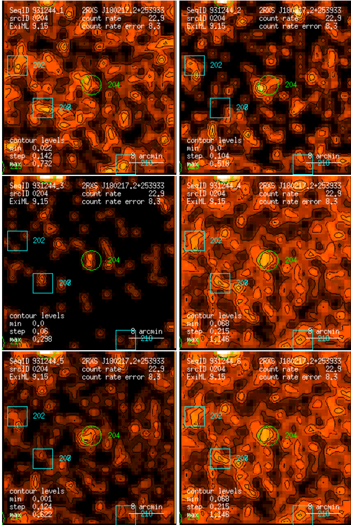
Figure 204: RASS 931244: detection 0204: band rate images, Gaussian filter: (1) PSPC channels 11 – 41, (2) 52 – 90, (3) 91 – 201, (4) 11 – 235, (5) 52 – 201, (6) 11 – 201. Broad band rates in counts/ks. Band rate contour levels in counts/ks/arcmin 2 .
