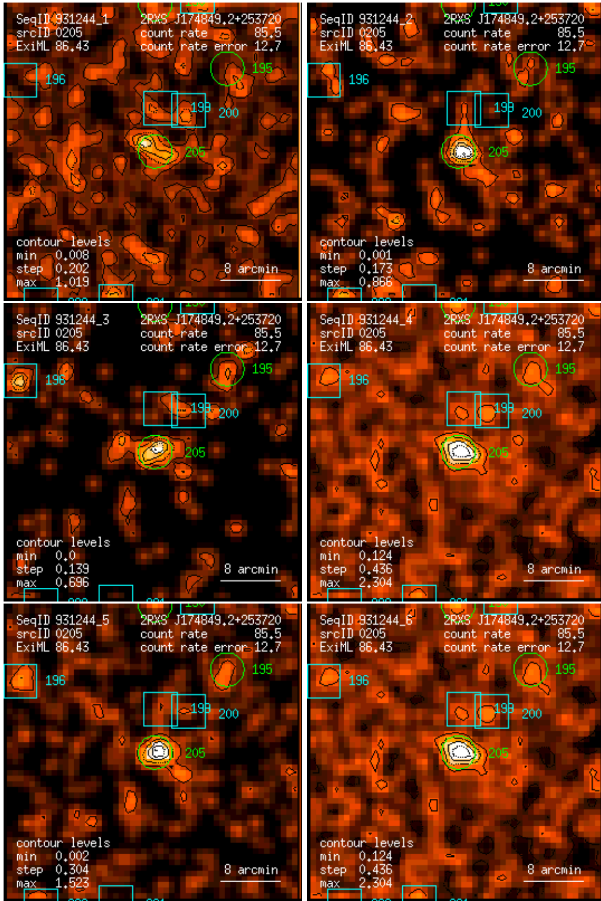
Figure 205: RASS 931244: detection 0205: band rate images, Gaussian filter: (1) PSPC channels 11 – 41, (2) 52 – 90, (3) 91 – 201, (4) 11 – 235, (5) 52 – 201, (6) 11 – 201. Broad band rates in counts/ks. Band rate contour levels in counts/ks/arcmin 2 .
