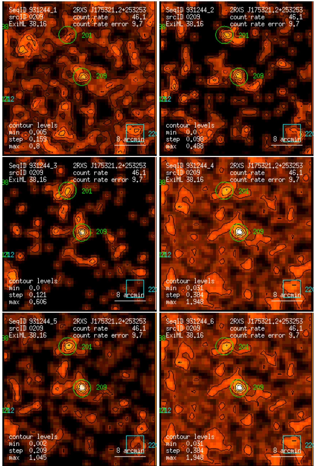
Figure 209: RASS 931244: detection 0209: band rate images, Gaussian filter: (1) PSPC channels 11 – 41, (2) 52 – 90, (3) 91 – 201, (4) 11 – 235, (5) 52 – 201, (6) 11 – 201. Broad band rates in counts/ks. Band rate contour levels in counts/ks/arcmin 2 .
