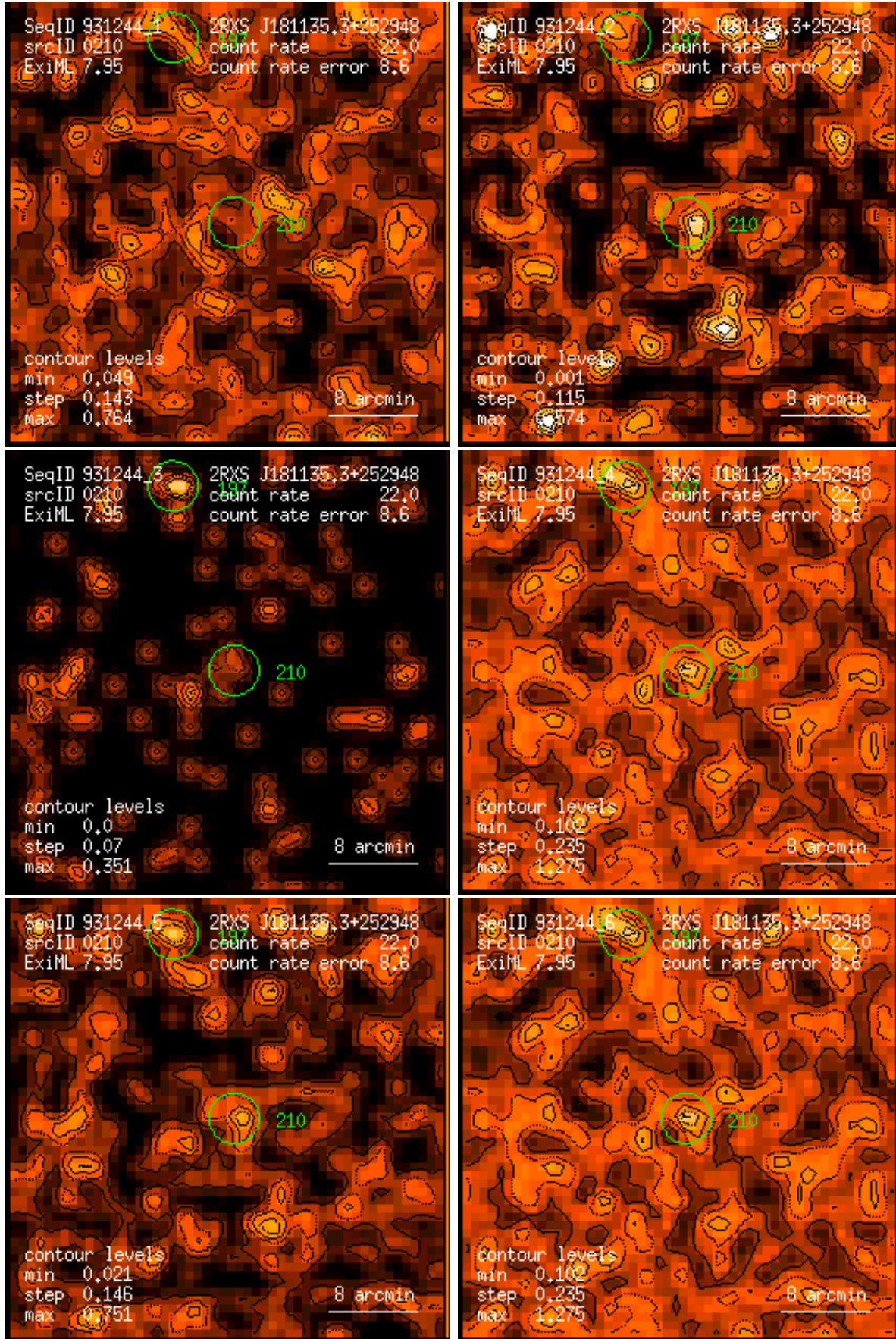
Figure 210: RASS 931244: detection 0210: band rate images, Gaussian filter: (1) PSPC channels 11 – 41, (2) 52 – 90, (3) 91 – 201, (4) 11 – 235, (5) 52 – 201, (6) 11 – 201. Broad band rates in counts/ks. Band rate contour levels in counts/ks/arcmin 2 .
