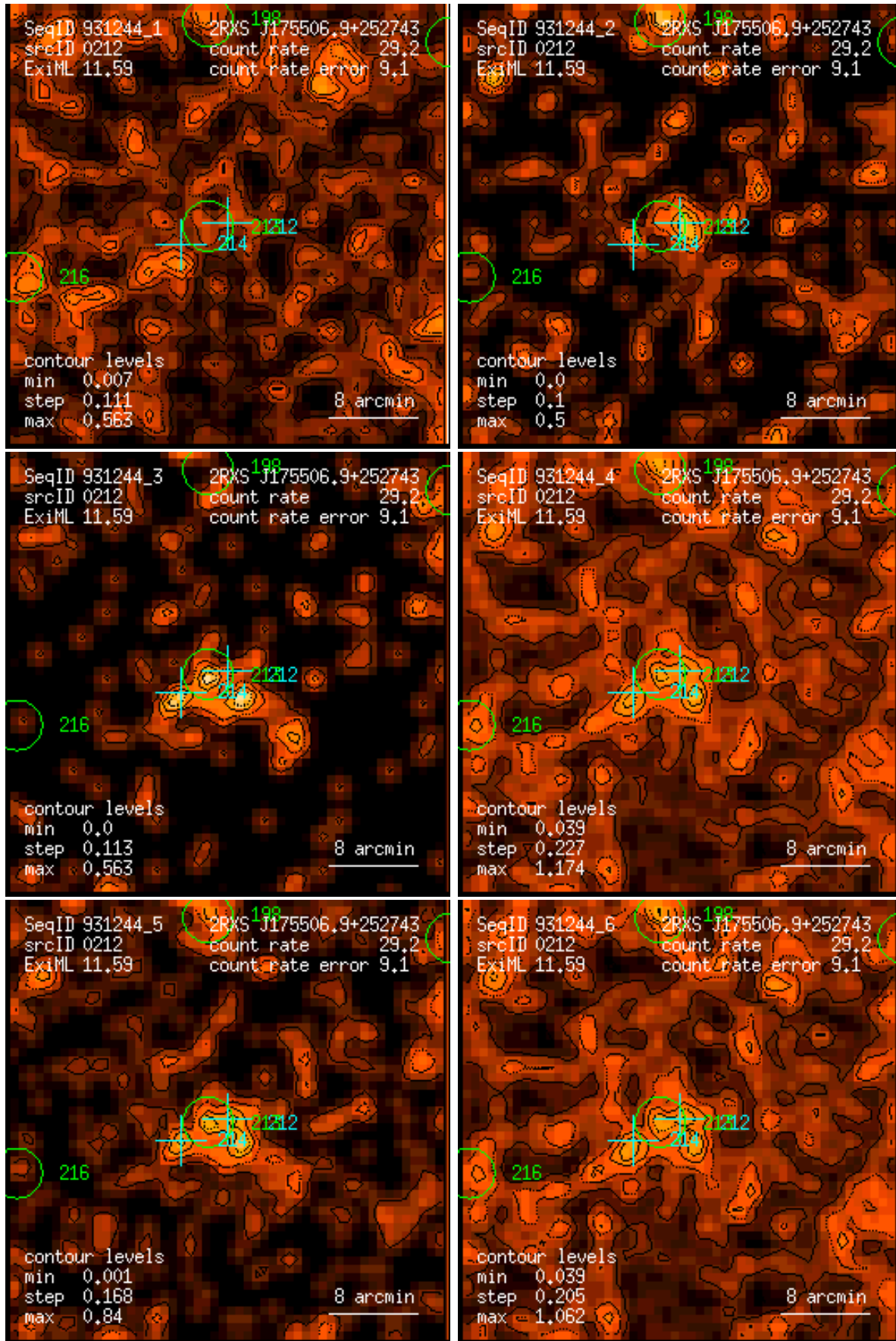
Figure 212: RASS 931244: detection 0212: band rate images, Gaussian filter: (1) PSPC channels 11 – 41, (2) 52 – 90, (3) 91 – 201, (4) 11 – 235, (5) 52 – 201, (6) 11 – 201. Broad band rates in counts/ks. Band rate contour levels in counts/ks/arcmin 2 .
