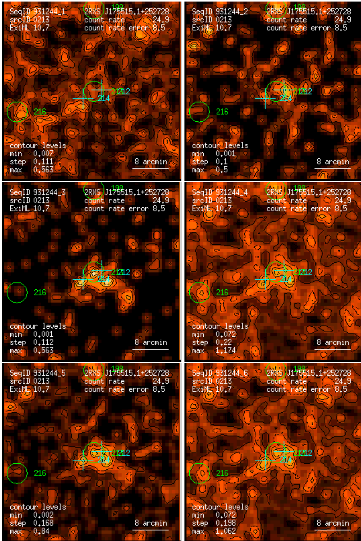
Figure 213: RASS 931244: detection 0213: band rate images, Gaussian filter: (1) PSPC channels 11 – 41, (2) 52 – 90, (3) 91 – 201, (4) 11 – 235, (5) 52 – 201, (6) 11 – 201. Broad band rates in counts/ks. Band rate contour levels in counts/ks/arcmin 2 .
