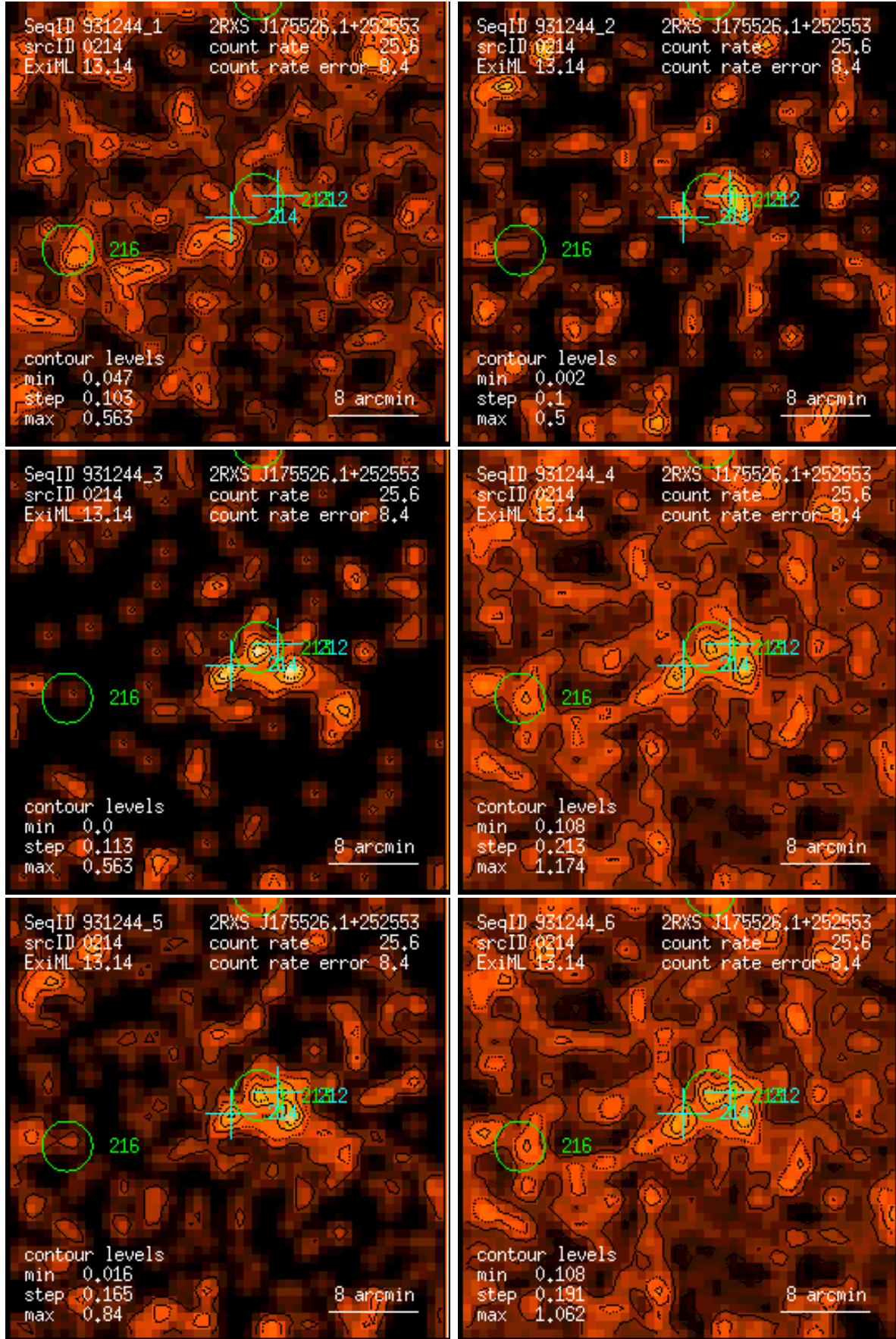
Figure 214: RASS 931244: detection 0214: band rate images, Gaussian filter: (1) PSPC channels 11 – 41, (2) 52 – 90, (3) 91 – 201, (4) 11 – 235, (5) 52 – 201, (6) 11 – 201. Broad band rates in counts/ks. Band rate contour levels in counts/ks/arcmin 2 .
