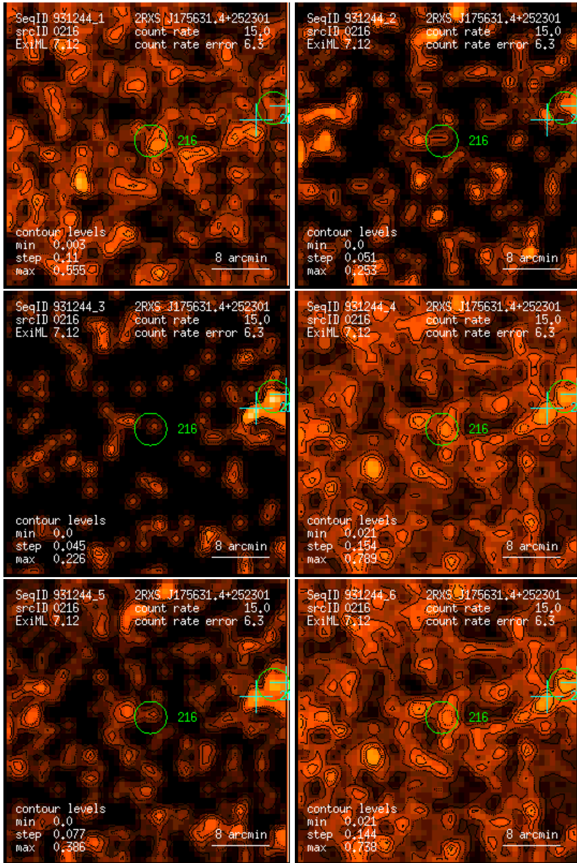
Figure 216: RASS 931244: detection 0216: band rate images, Gaussian filter: (1) PSPC channels 11 – 41, (2) 52 – 90, (3) 91 – 201, (4) 11 – 235, (5) 52 – 201, (6) 11 – 201. Broad band rates in counts/ks. Band rate contour levels in counts/ks/arcmin 2 .
