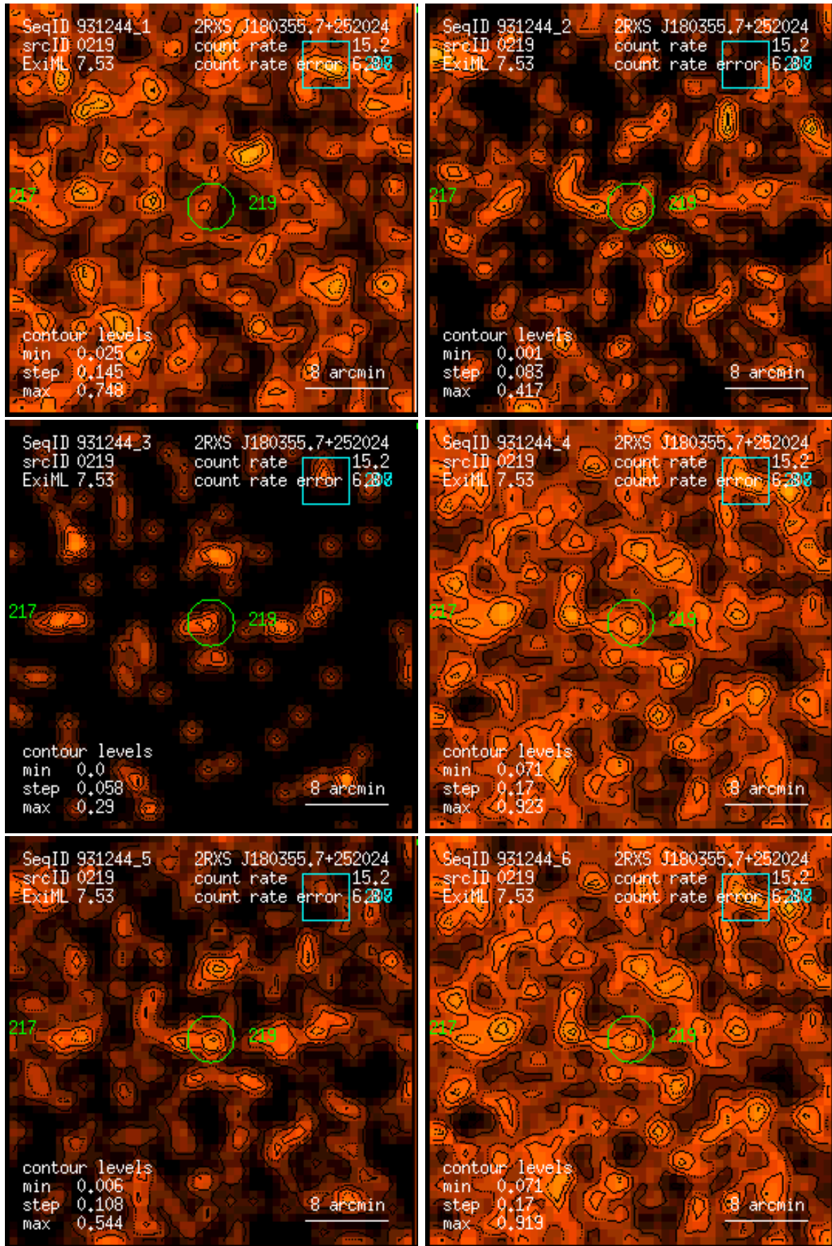
Figure 219: RASS 931244: detection 0219: band rate images, Gaussian filter: (1) PSPC channels 11 – 41, (2) 52 – 90, (3) 91 – 201, (4) 11 – 235, (5) 52 – 201, (6) 11 – 201. Broad band rates in counts/ks. Band rate contour levels in counts/ks/arcmin 2 .
