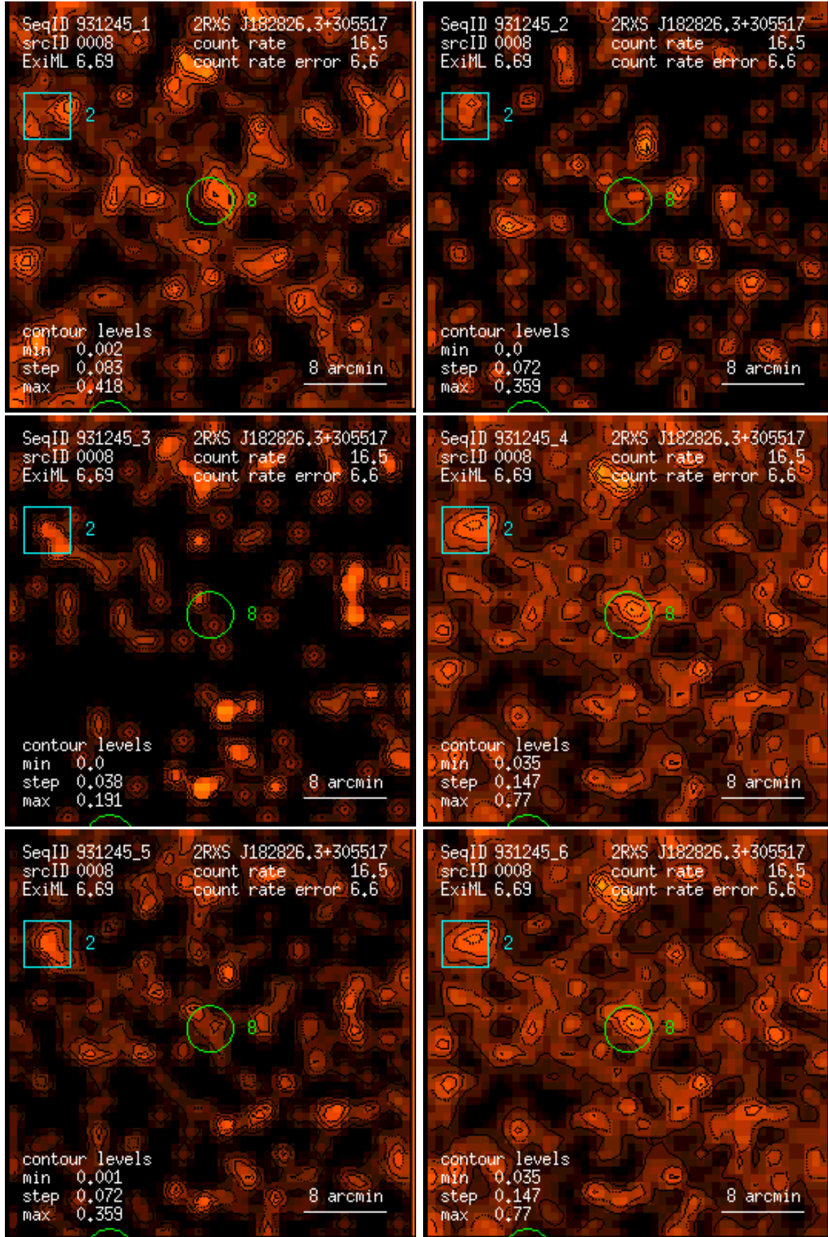
Figure 8: RASS 931245: detection 0008: band rate images, Gaussian filter: (1) PSPC channels 11 – 41, (2) 52 – 90, (3) 91 – 201, (4) 11 – 235, (5) 52 – 201, (6) 11 – 201. Broad band rates in counts/ks. Band rate contour levels in counts/ks/arcmin 2 .
