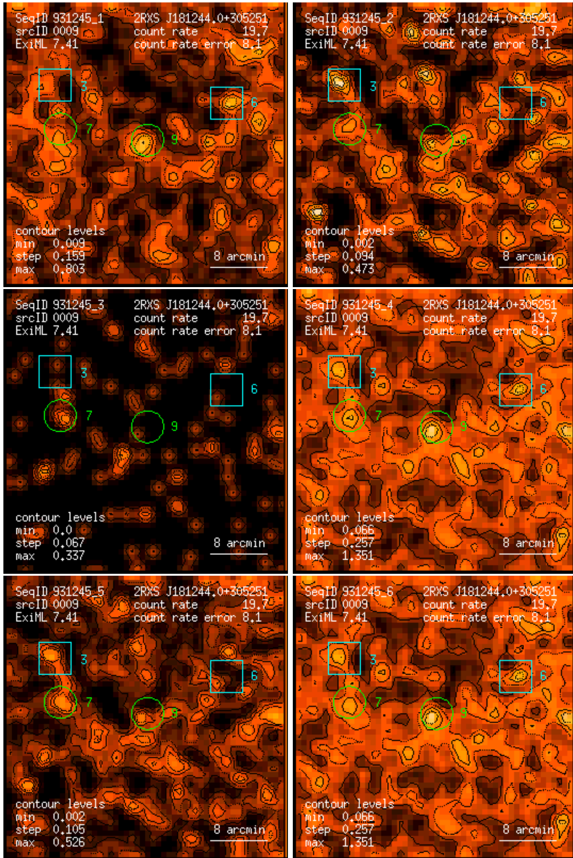
Figure 9: RASS 931245: detection 0009: band rate images, Gaussian filter: (1) PSPC channels 11 – 41, (2) 52 – 90, (3) 91 – 201, (4) 11 – 235, (5) 52 – 201, (6) 11 – 201. Broad band rates in counts/ks. Band rate contour levels in counts/ks/arcmin 2 .
