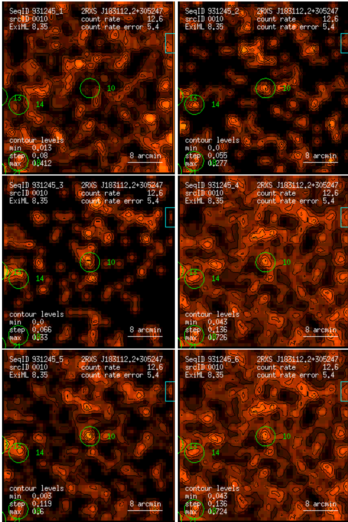
Figure 10: RASS 931245: detection 0010: band rate images, Gaussian filter: (1) PSPC channels 11 – 41, (2) 52 – 90, (3) 91 – 201, (4) 11 – 235, (5) 52 – 201, (6) 11 – 201. Broad band rates in counts/ks. Band rate contour levels in counts/ks/arcmin 2 .
