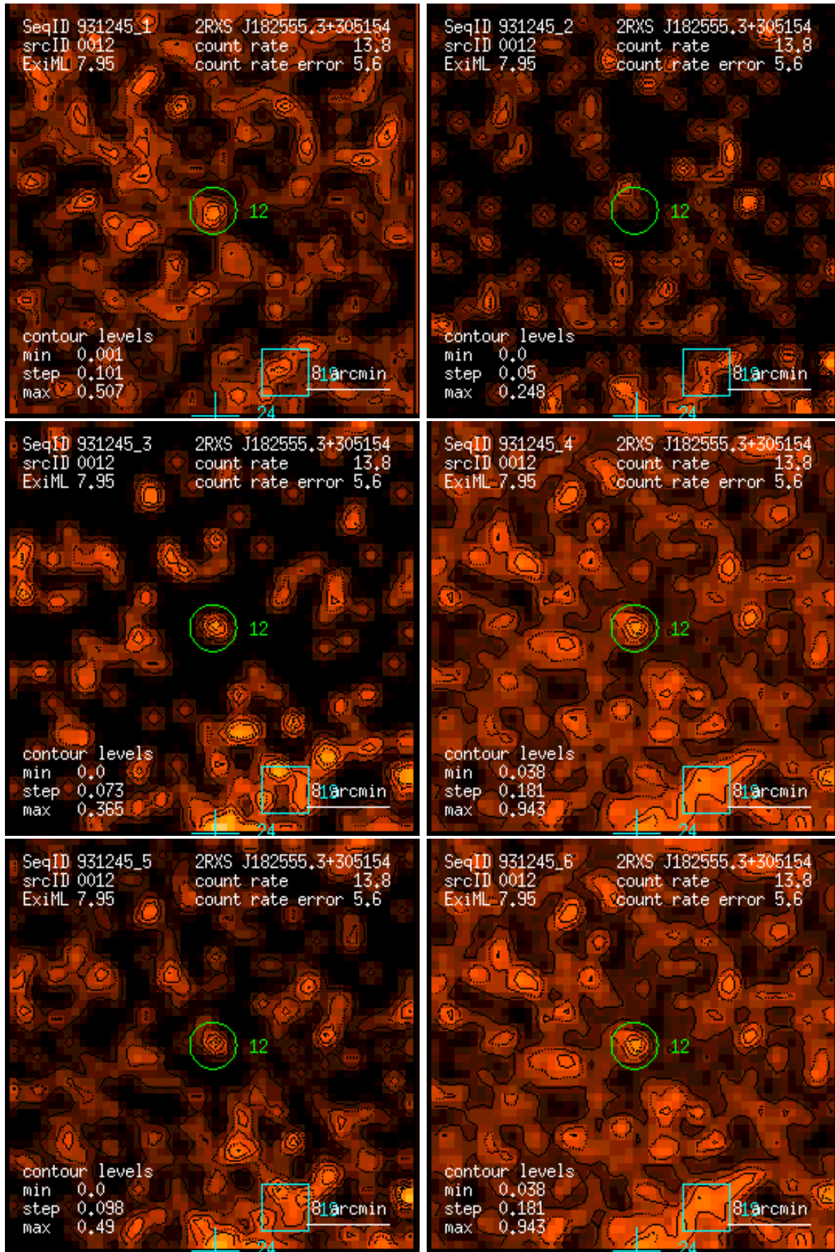
Figure 12: RASS 931245: detection 0012: band rate images, Gaussian filter: (1) PSPC channels 11 – 41, (2) 52 – 90, (3) 91 – 201, (4) 11 – 235, (5) 52 – 201, (6) 11 – 201. Broad band rates in counts/ks. Band rate contour levels in counts/ks/arcmin 2 .
