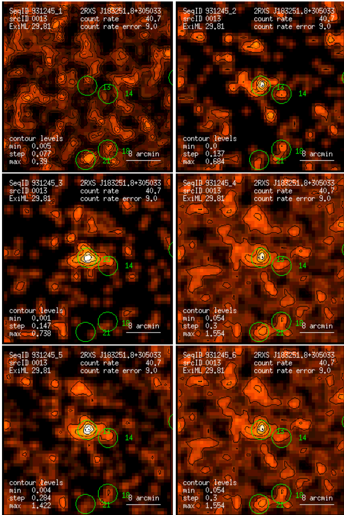
Figure 13: RASS 931245: detection 0013: band rate images, Gaussian filter: (1) PSPC channels 11 – 41, (2) 52 – 90, (3) 91 – 201, (4) 11 – 235, (5) 52 – 201, (6) 11 – 201. Broad band rates in counts/ks. Band rate contour levels in counts/ks/arcmin 2 .
