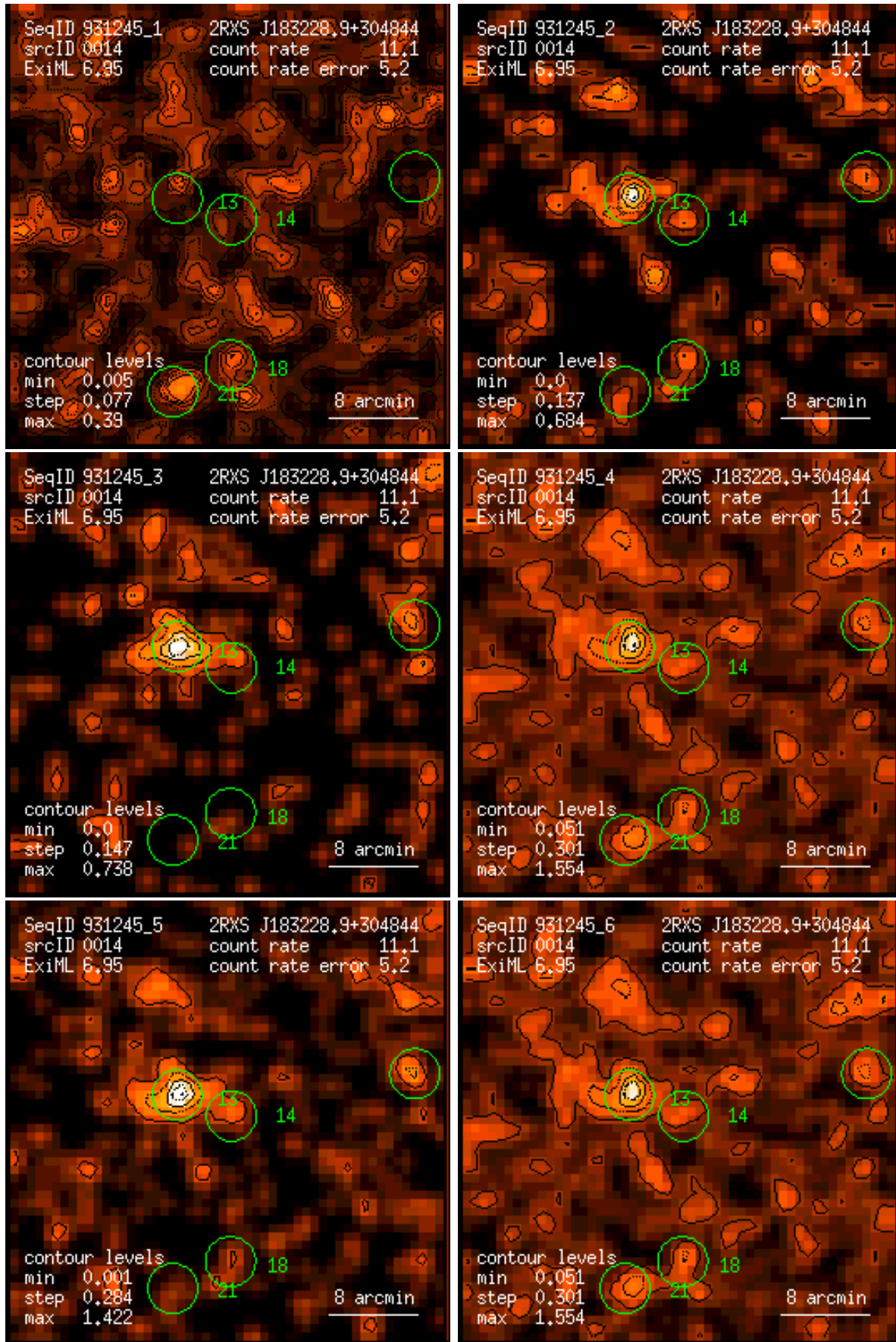
Figure 14: RASS 931245: detection 0014: band rate images, Gaussian filter: (1) PSPC channels 11 – 41, (2) 52 – 90, (3) 91 – 201, (4) 11 – 235, (5) 52 – 201, (6) 11 – 201. Broad band rates in counts/ks. Band rate contour levels in counts/ks/arcmin 2 .
