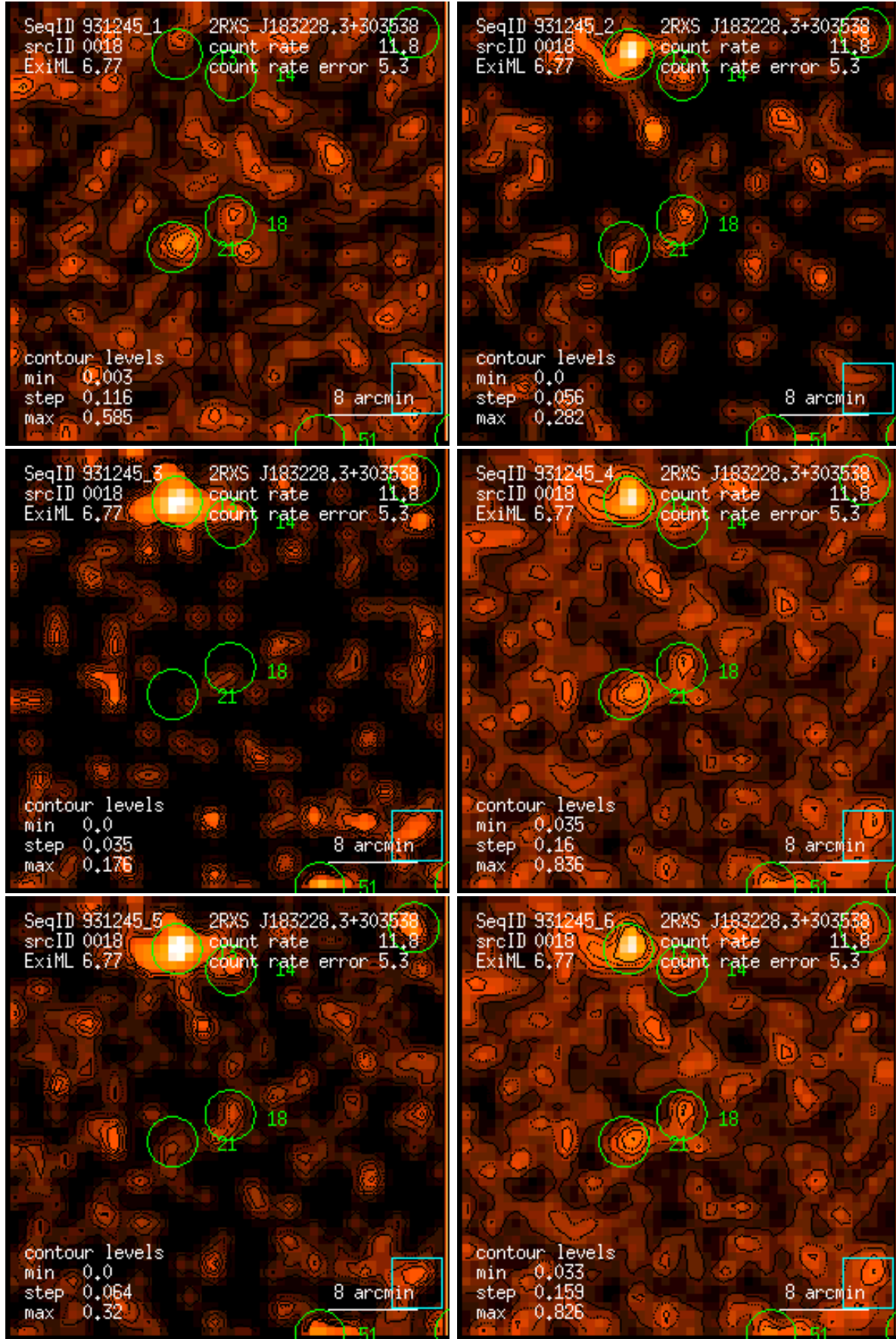
Figure 18: RASS 931245: detection 0018: band rate images, Gaussian filter: (1) PSPC channels 11 – 41, (2) 52 – 90, (3) 91 – 201, (4) 11 – 235, (5) 52 – 201, (6) 11 – 201. Broad band rates in counts/ks. Band rate contour levels in counts/ks/arcmin 2 .
