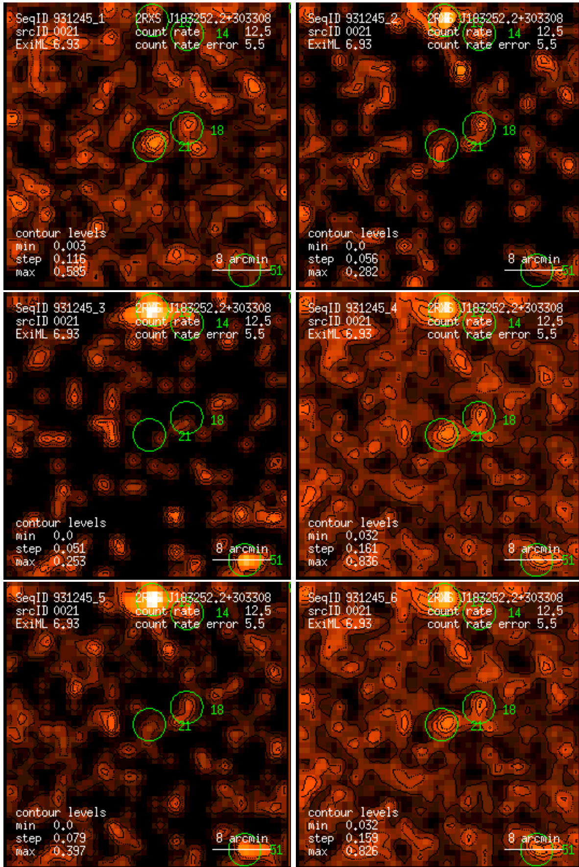
Figure 21: RASS 931245: detection 0021: band rate images, Gaussian filter: (1) PSPC channels 11 – 41, (2) 52 – 90, (3) 91 – 201, (4) 11 – 235, (5) 52 – 201, (6) 11 – 201. Broad band rates in counts/ks. Band rate contour levels in counts/ks/arcmin 2 .
