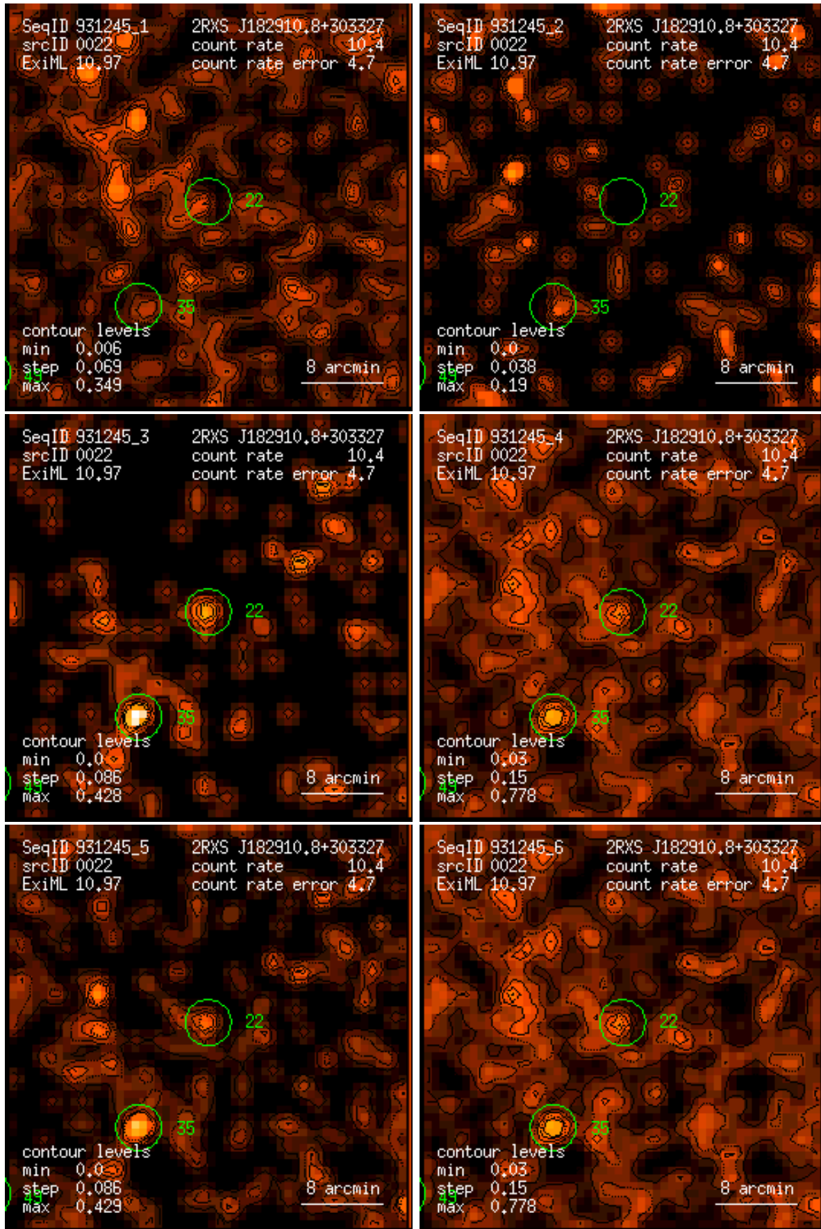
Figure 22: RASS 931245: detection 0022: band rate images, Gaussian filter: (1) PSPC channels 11 – 41, (2) 52 – 90, (3) 91 – 201, (4) 11 – 235, (5) 52 – 201, (6) 11 – 201. Broad band rates in counts/ks. Band rate contour levels in counts/ks/arcmin 2 .
