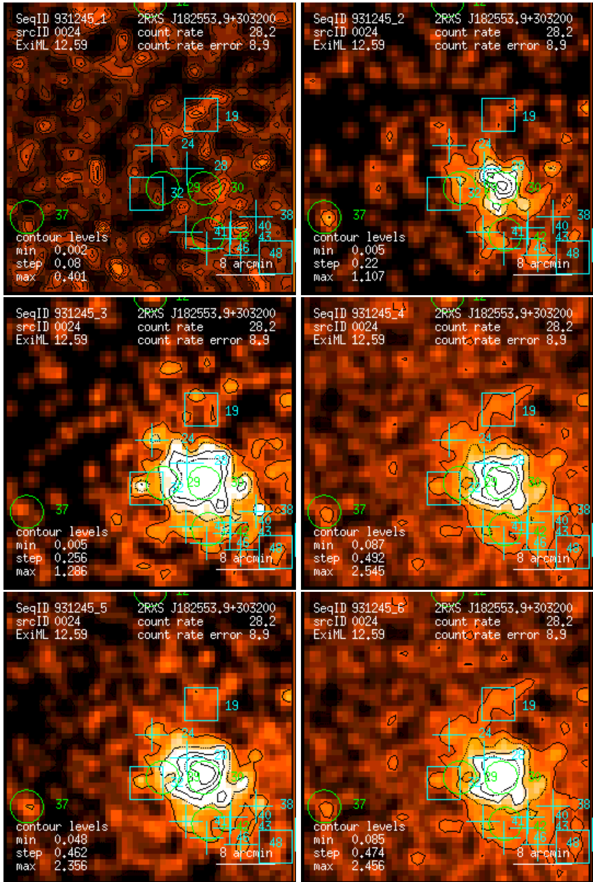
Figure 24: RASS 931245: detection 0024: band rate images, Gaussian filter: (1) PSPC channels 11 – 41, (2) 52 – 90, (3) 91 – 201, (4) 11 – 235, (5) 52 – 201, (6) 11 – 201. Broad band rates in counts/ks. Band rate contour levels in counts/ks/arcmin 2 .
