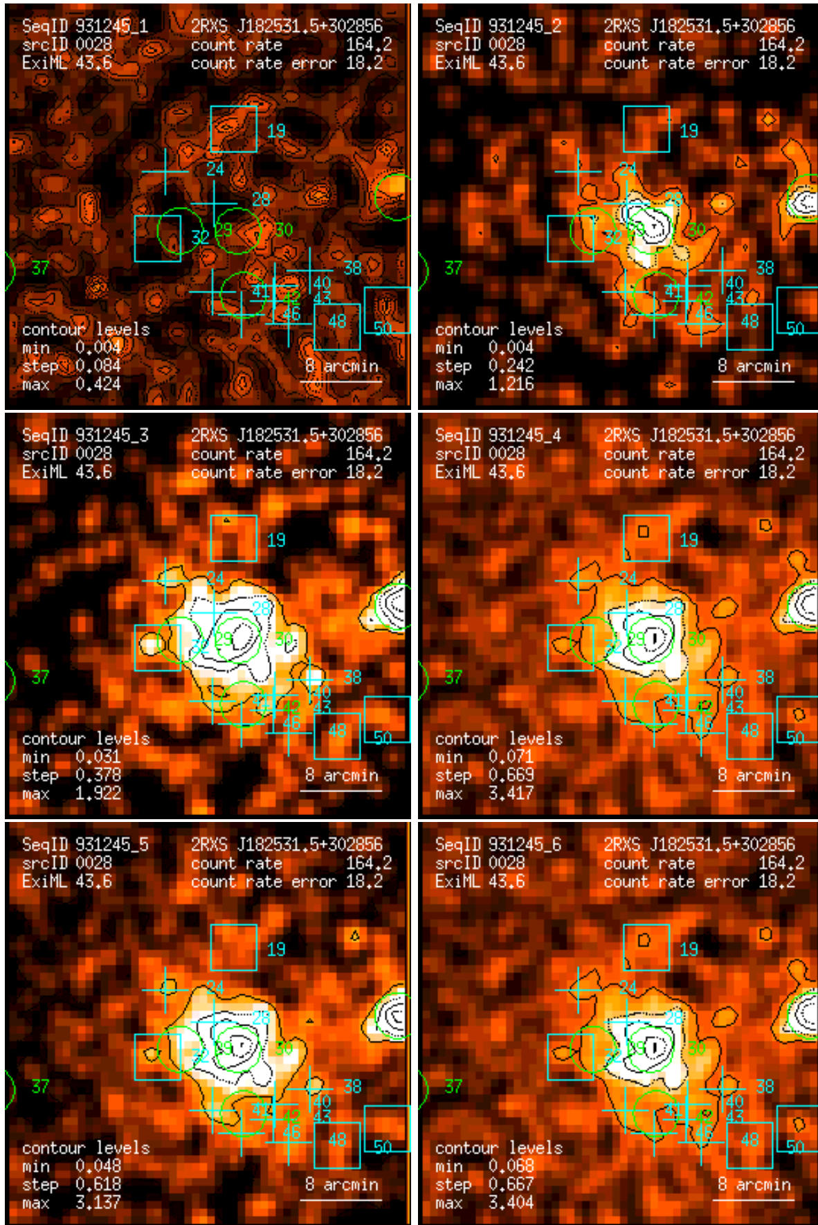
Figure 28: RASS 931245: detection 0028: band rate images, Gaussian filter: (1) PSPC channels 11 – 41, (2) 52 – 90, (3) 91 – 201, (4) 11 – 235, (5) 52 – 201, (6) 11 – 201. Broad band rates in counts/ks. Band rate contour levels in counts/ks/arcmin 2 .
