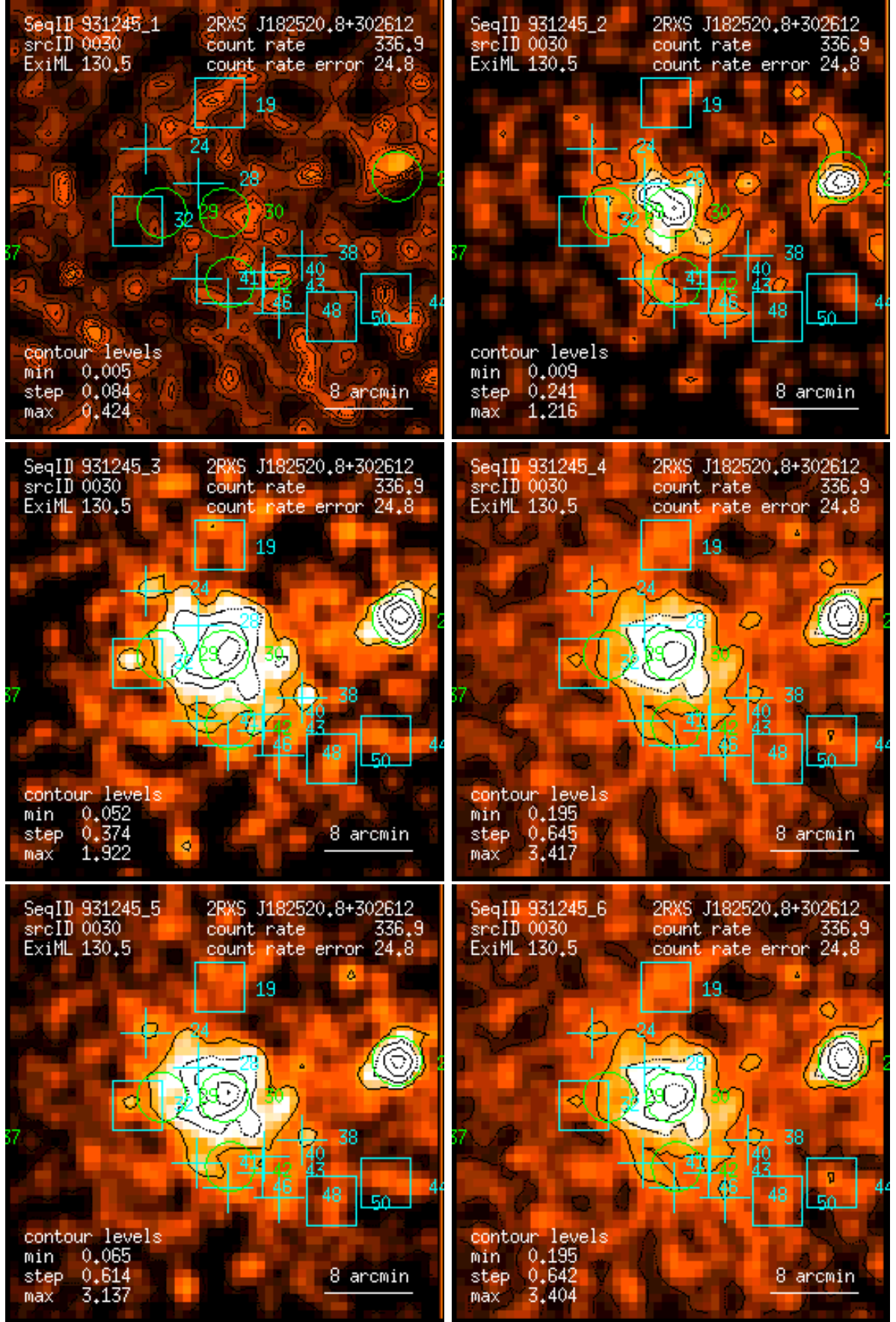
Figure 30: RASS 931245: detection 0030: band rate images, Gaussian filter: (1) PSPC channels 11 – 41, (2) 52 – 90, (3) 91 – 201, (4) 11 – 235, (5) 52 – 201, (6) 11 – 201. Broad band rates in counts/ks. Band rate contour levels in counts/ks/arcmin 2 .
